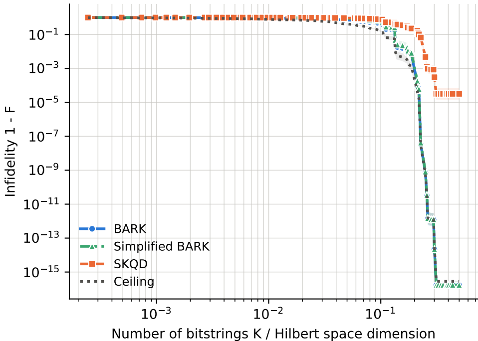
runs per point -- BARK: 76-283, Ceiling: 76-283, SKQD: 76-283, Simplified BARK: 76-283
