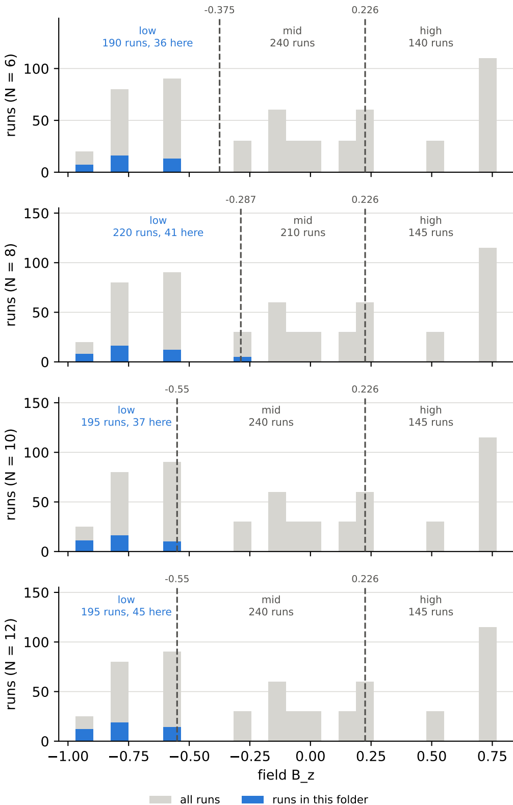
field B_z over all runs, and the cuts behind the bins lattice dimension = 2, field B_z = low, initial overlap = high
