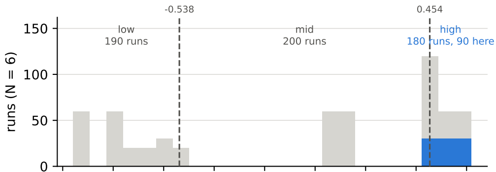
coupling J over all runs, and the cuts behind the bins lattice dimension = 2, coupling J = high
