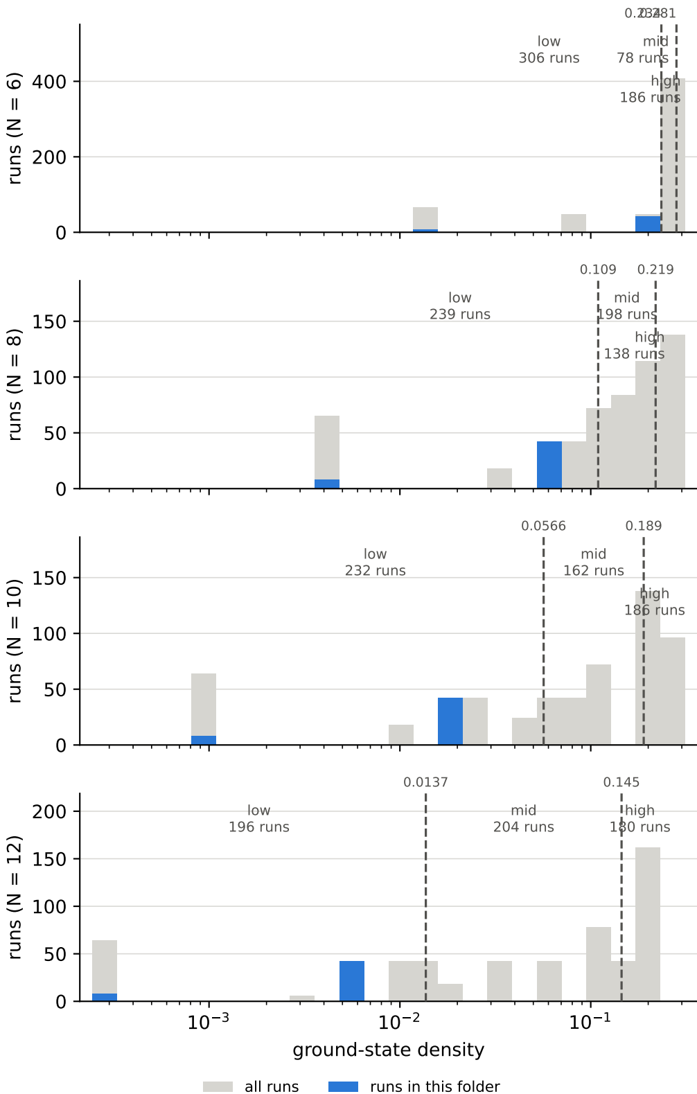
ground-state density over all runs, and the cuts behind the bins lattice dimension = 1, anisotropy \delta = 100
