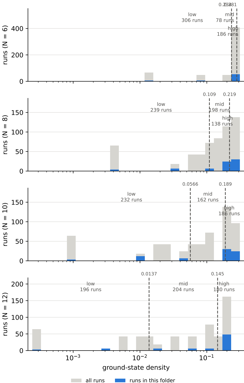
ground-state density over all runs, and the cuts behind the bins lattice dimension = 2, anisotropy \delta = 0.5
