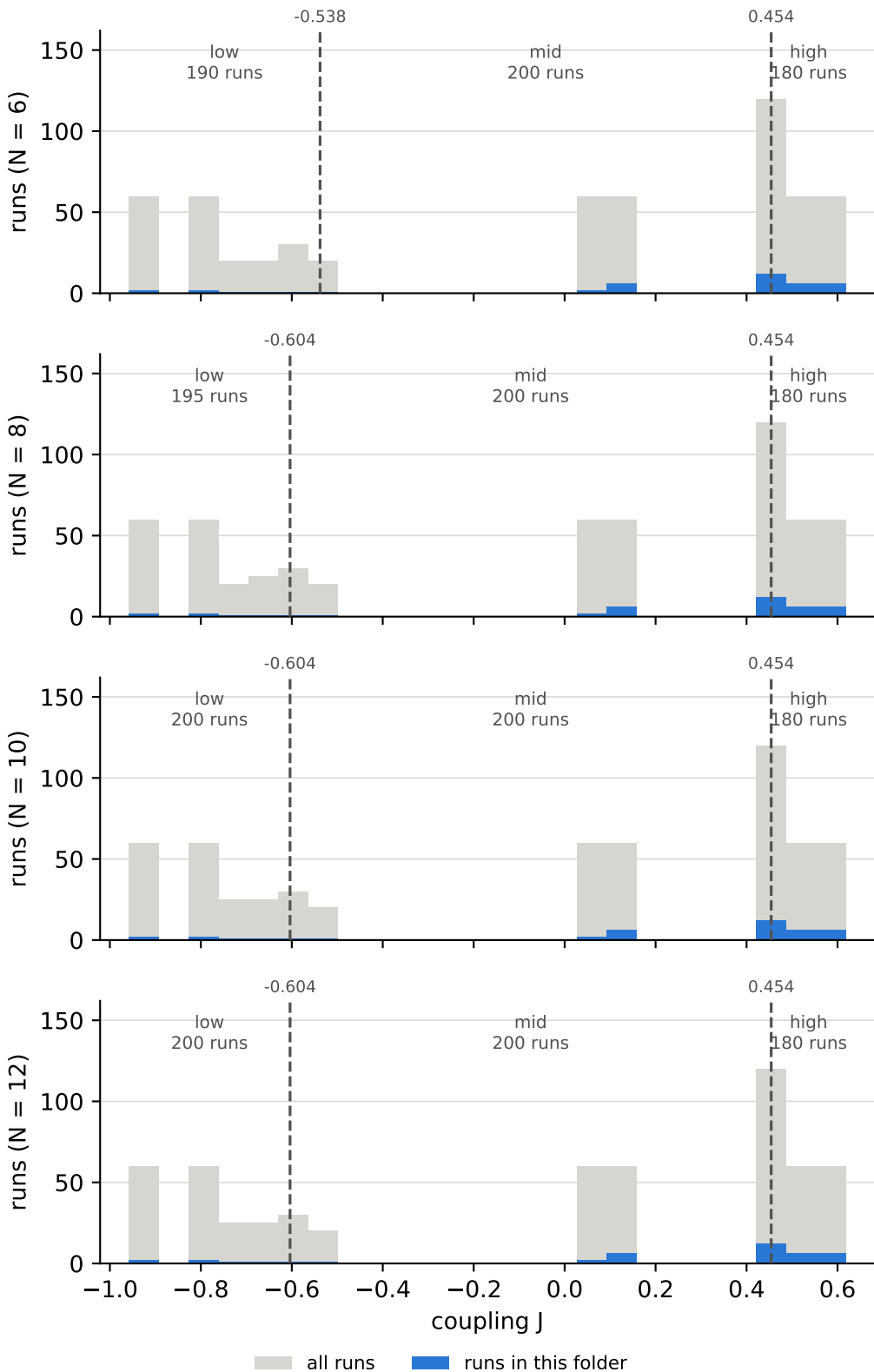
coupling J over all runs, and the cuts behind the bins lattice dimension = 2, anisotropy \delta = 1
