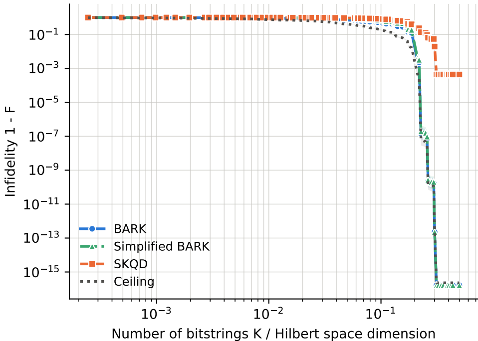
runs per point -- BARK: 129-443, Ceiling: 129-443, SKQD: 129-443, Simplified BARK: 129-443
