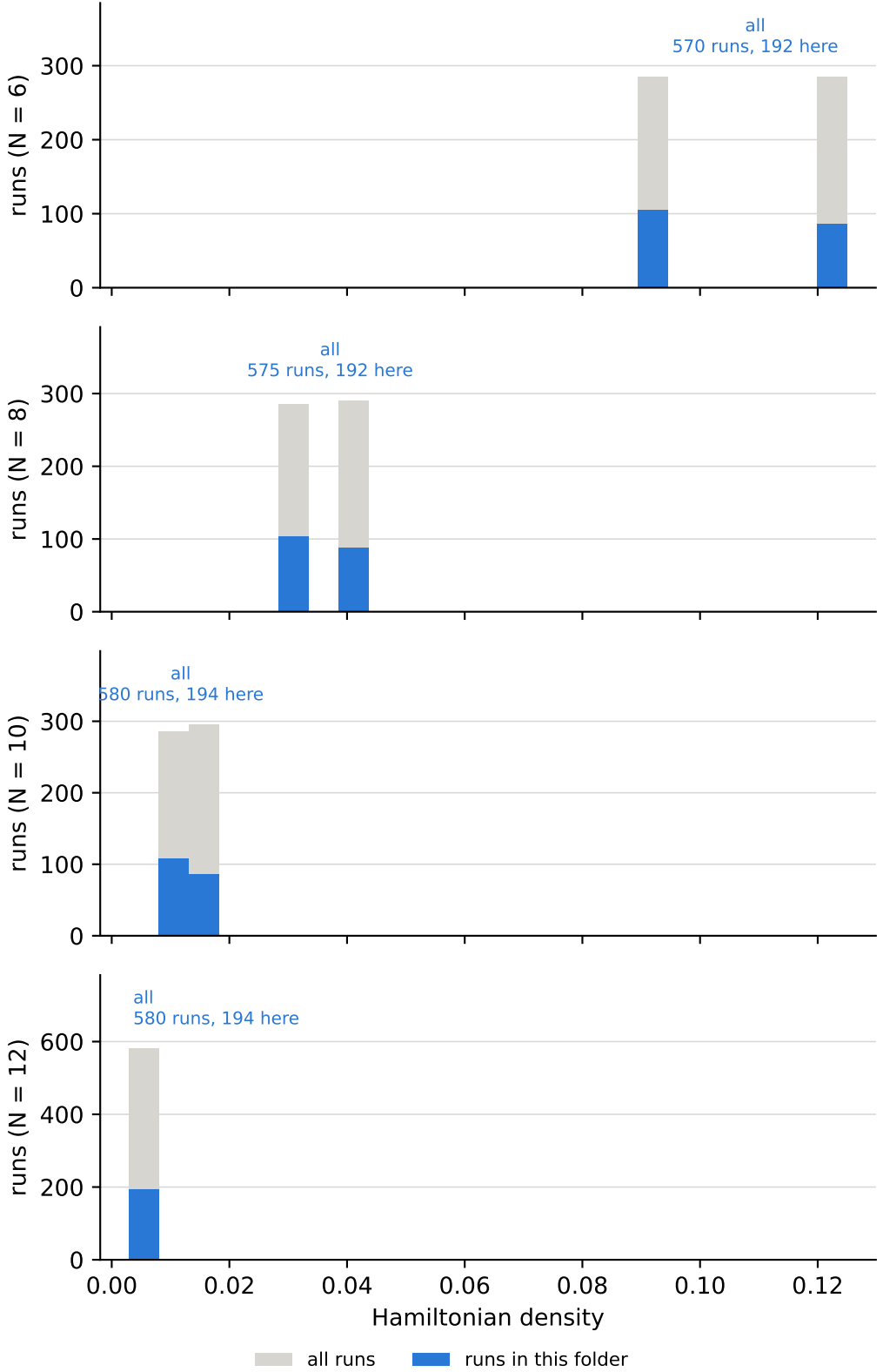
Hamiltonian density over all runs, and the cuts behind the bins Hamiltonian density = all, initial overlap = low
