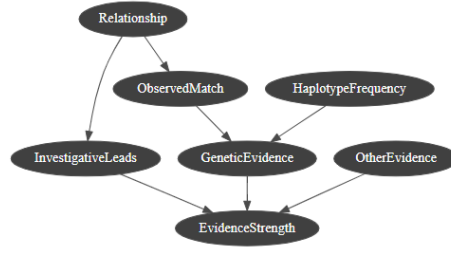
Figure 1: Resulting Bayesian network.
