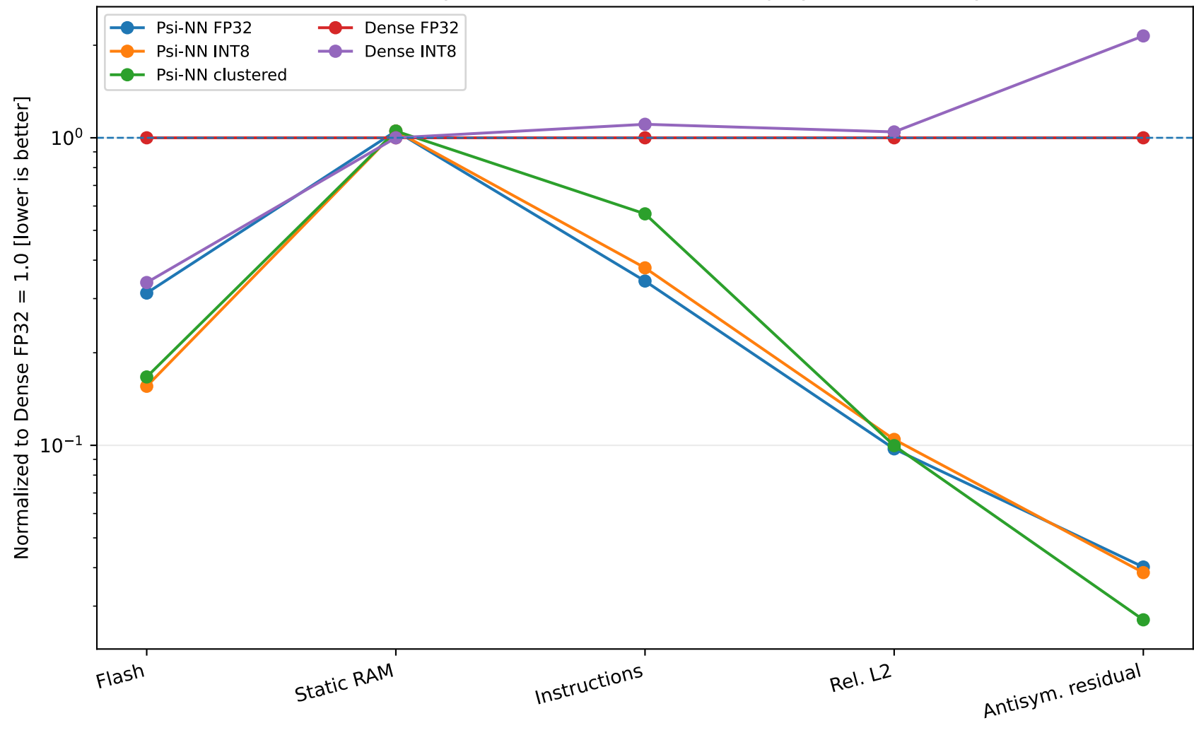
Linked-binary and emulated Cortex-M deployment summary
