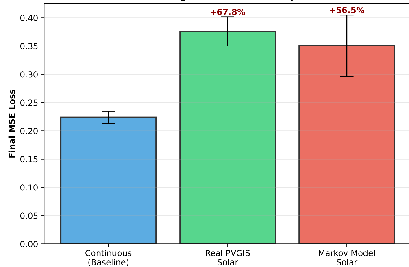
(c) Training Performance Comparison
