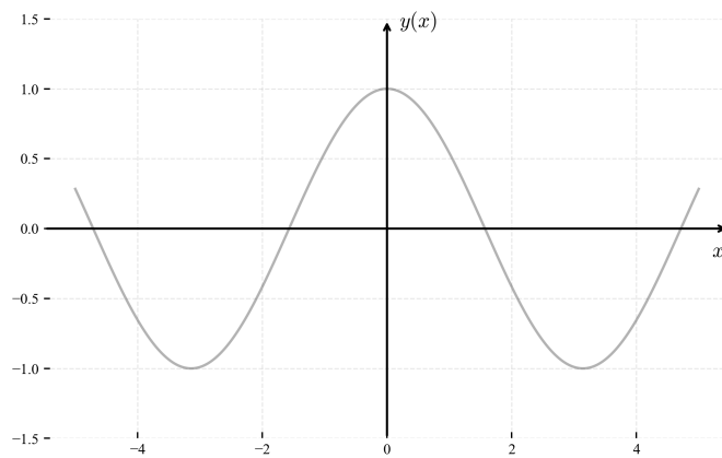
(c) Representation of a sinusoidal function y(x) = a \sin(x) + b \cos(x) . Example of these are, for instance, the position of a wire with respect to time in a harmonic movement x(t) = A \cos(\omega t + \phi) .
