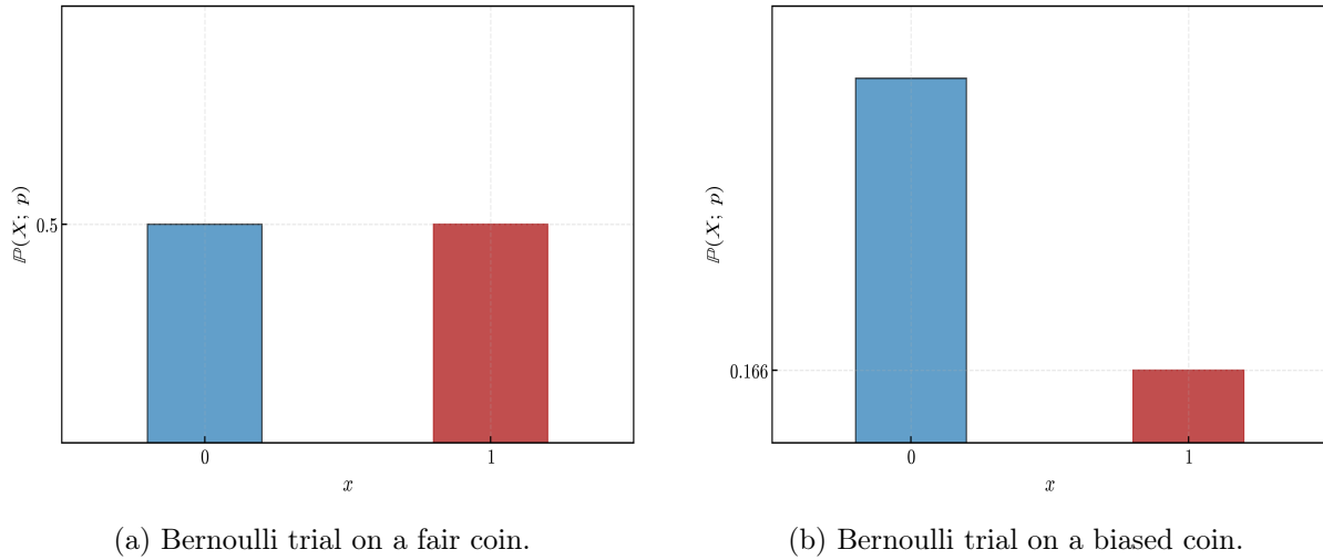
Figure 2.1: Bernoulli probability mass distribution.
