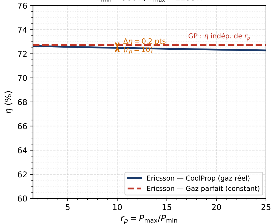
Influence de r_p T_{\min} = 300 \text{ K} , T_{\max} = 1100 \text{ K}
