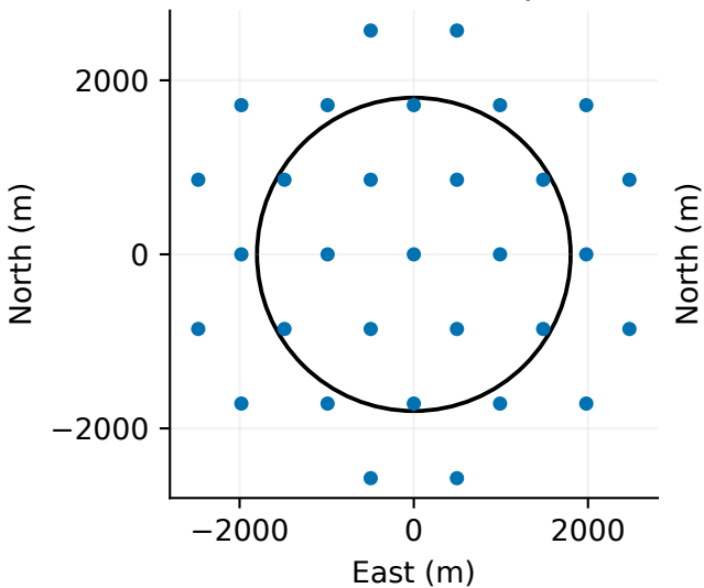
Control: 31 lattice points
