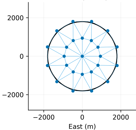
Refined: 25 polar points
