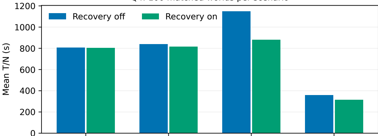
Q4: 100 matched worlds per scenario
