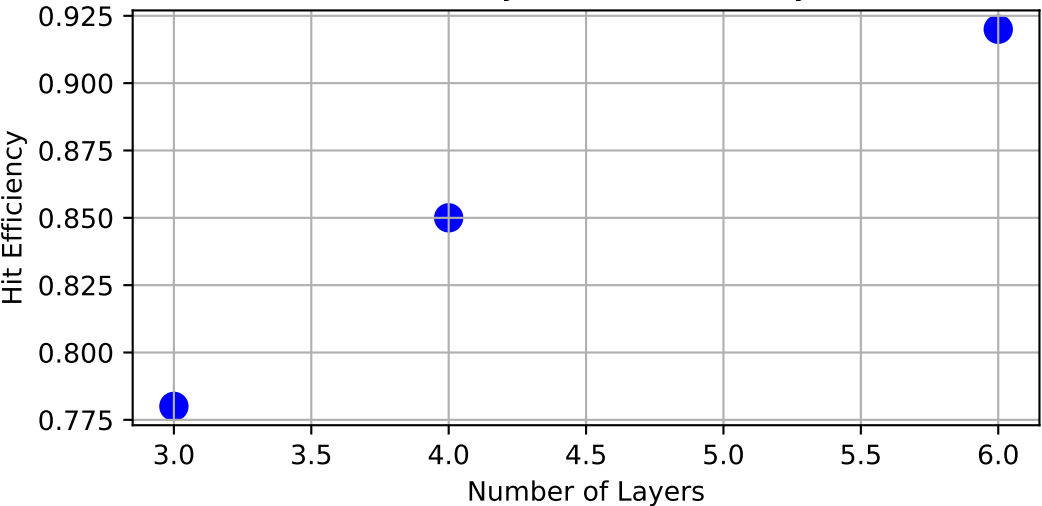
Hit Efficiency vs Number of Layers
