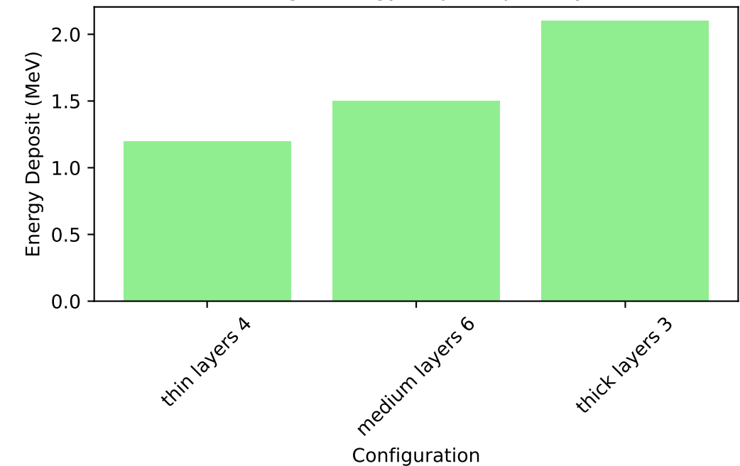
Average Energy Deposit per Layer
