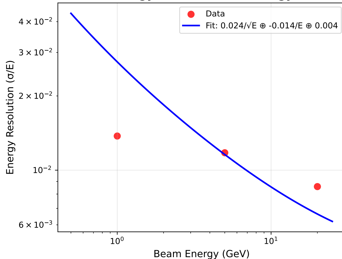
Energy Resolution vs Energy
