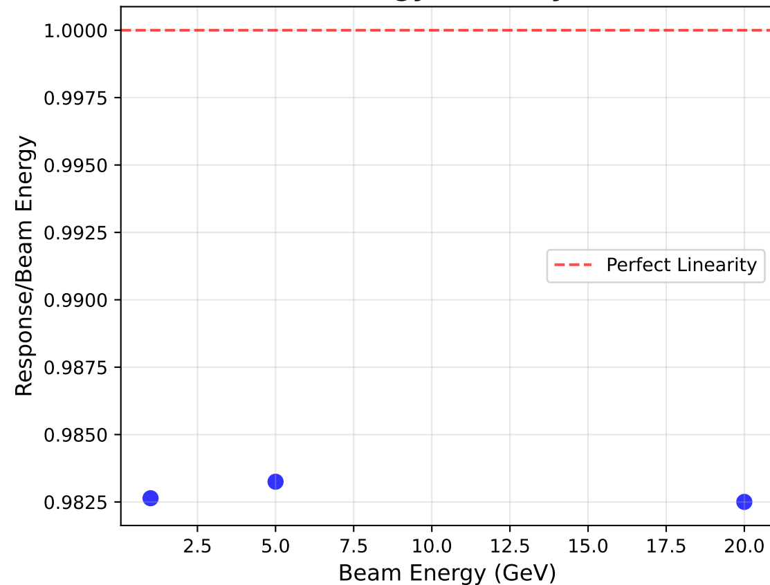
Energy Linearity
