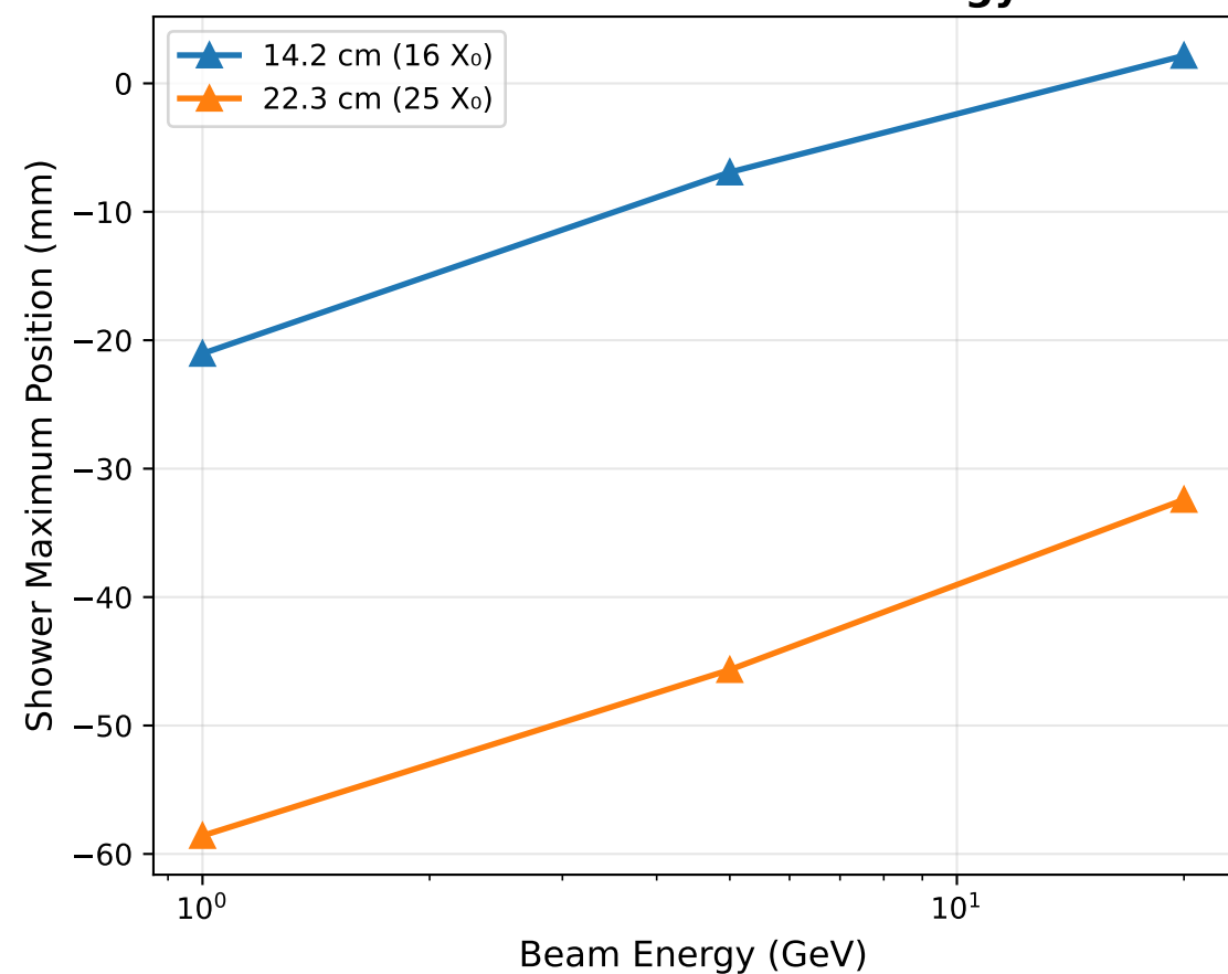
Shower Maximum vs Energy
