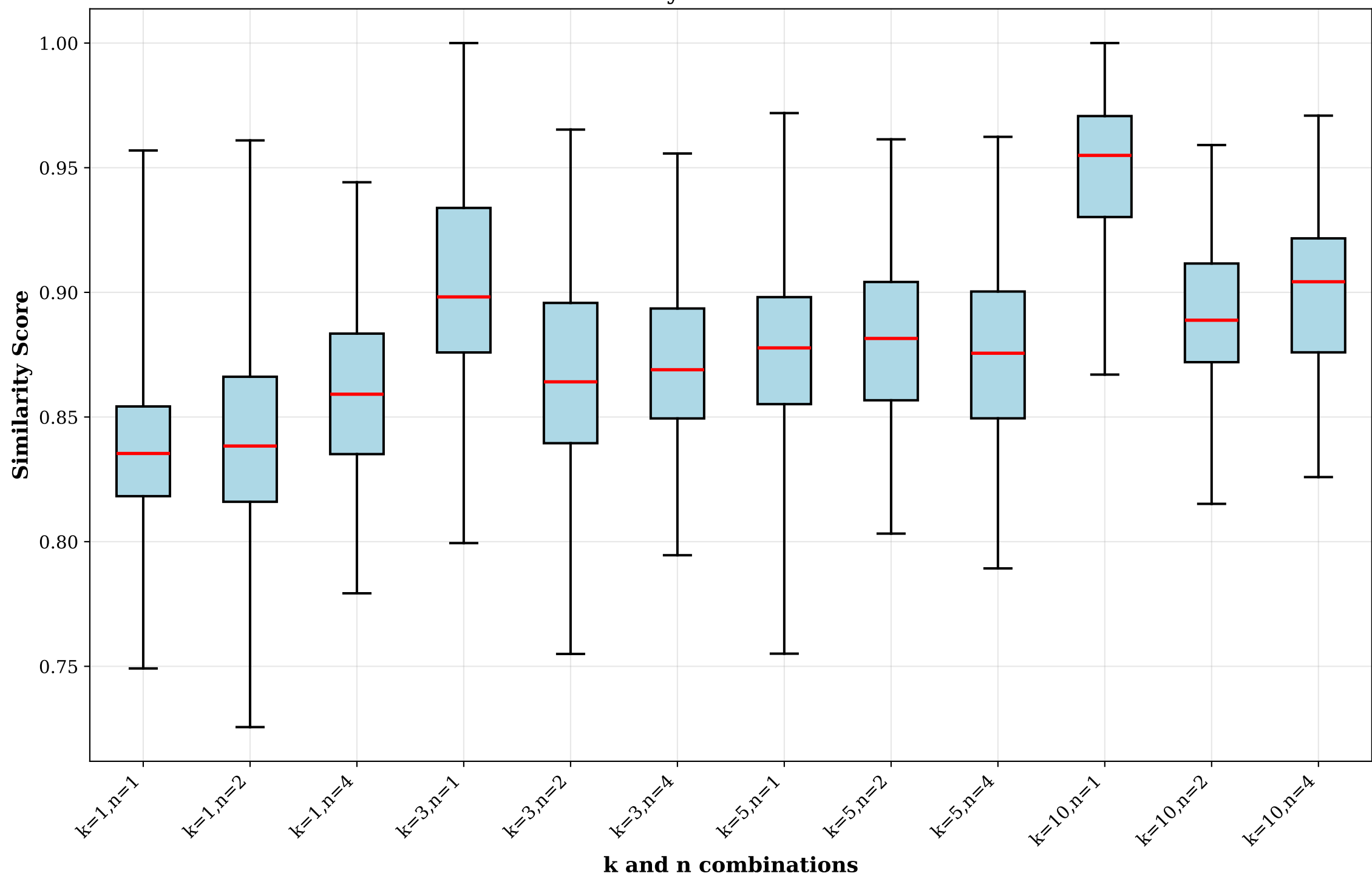
Similarity Trends for c=200
