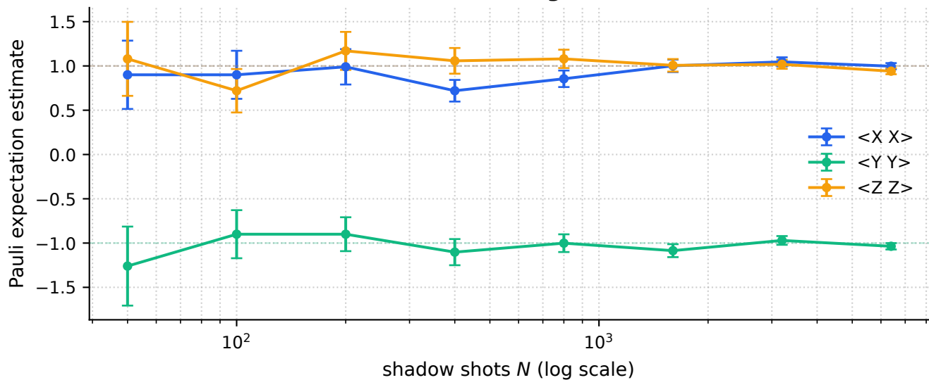
Pauli classical shadow convergence on the Bell state
