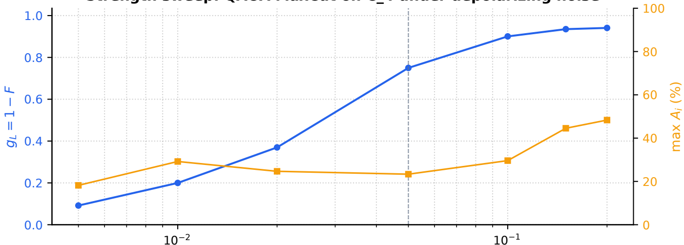
Strength sweep: QAOA MaxCut on C 4 under depolarizing noise
