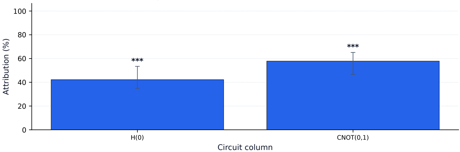
Pauli-twirled (same circuit, same noise)
