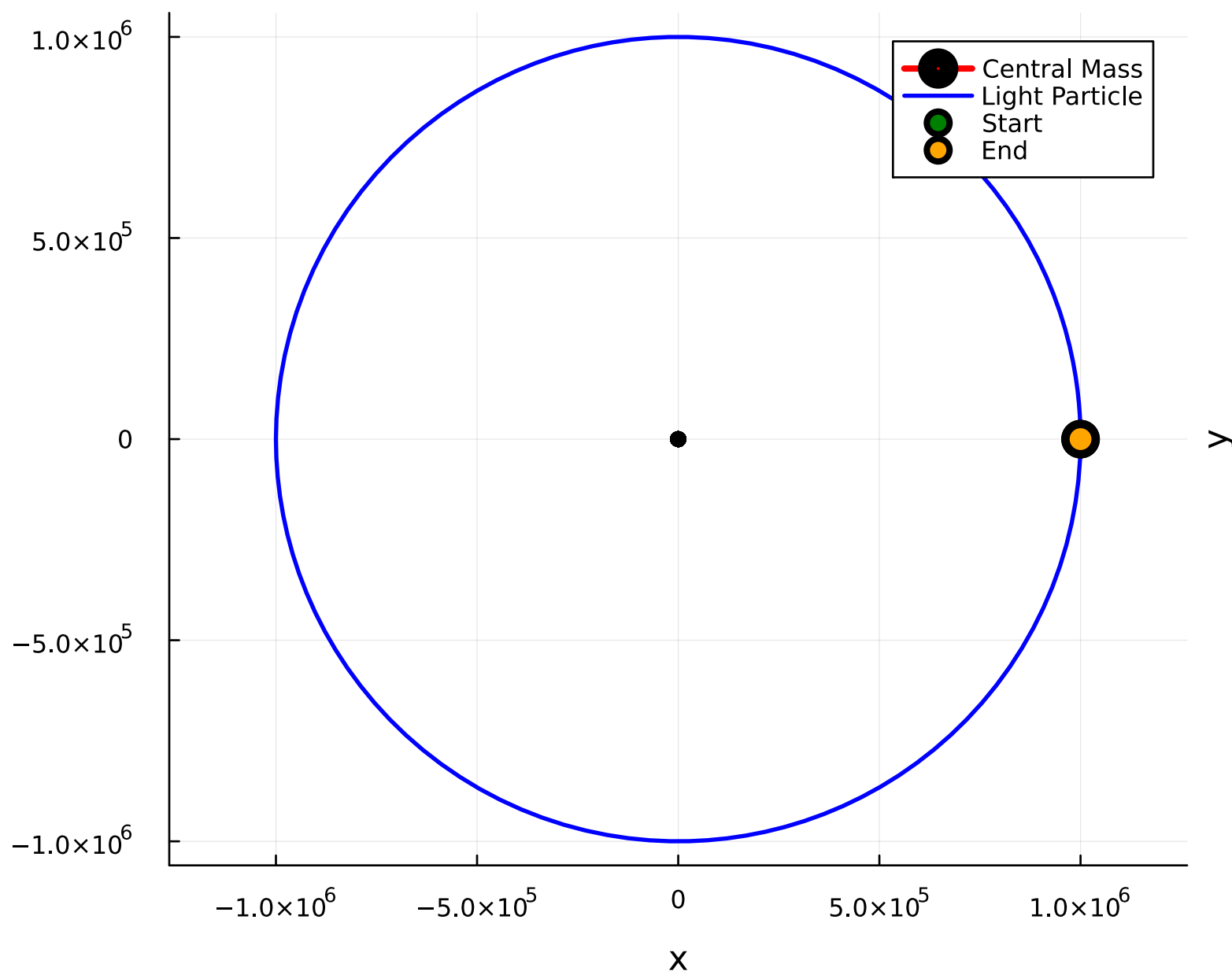
Test Particle Orbital Motion
