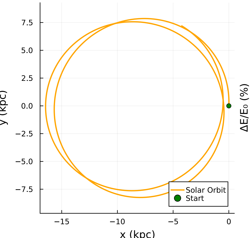
Solar Orbit
