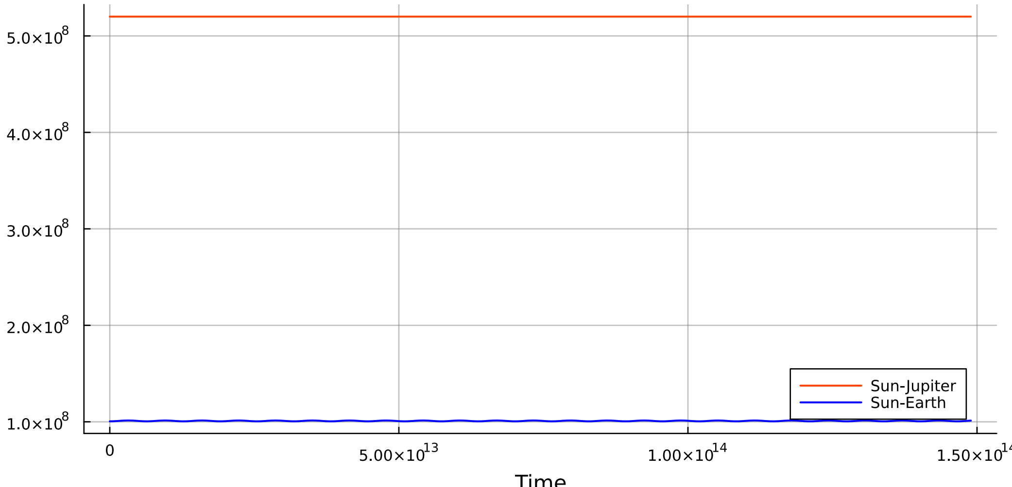
Separation in Sun-Jupiter-(test)_Earth System
