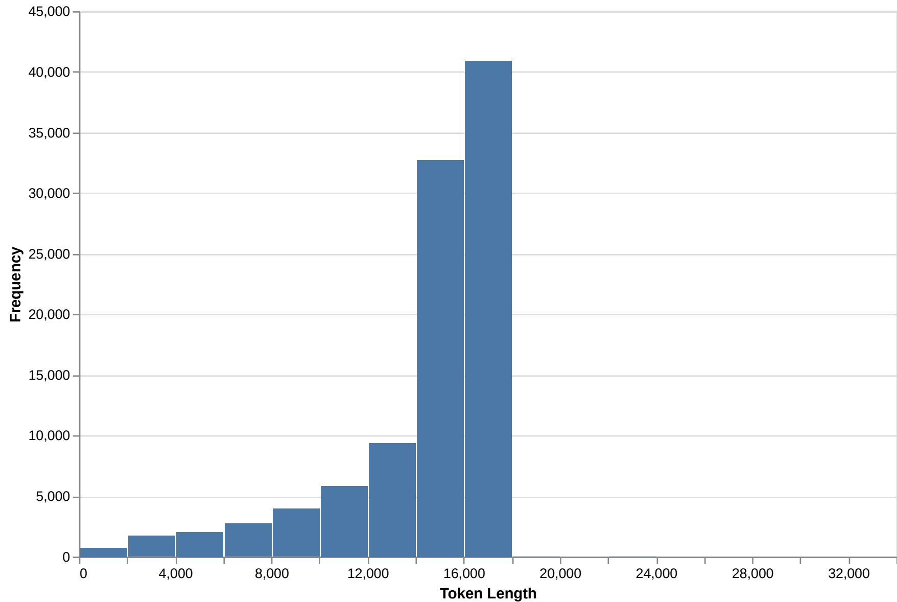
Distribution of Solution Token Lengths
