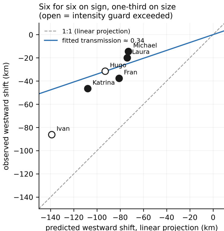
Fig. 3. Observed westward cross-track shift versus the strong-form (linear) projection for the six-storm A/B. Every storm moves west, as predicted; the fitted transmission is \approx 0.34 of the linear projection (dashed line: 1:1). Open symbols mark the two intensity-guard exceedances, excluded from the estimate.
