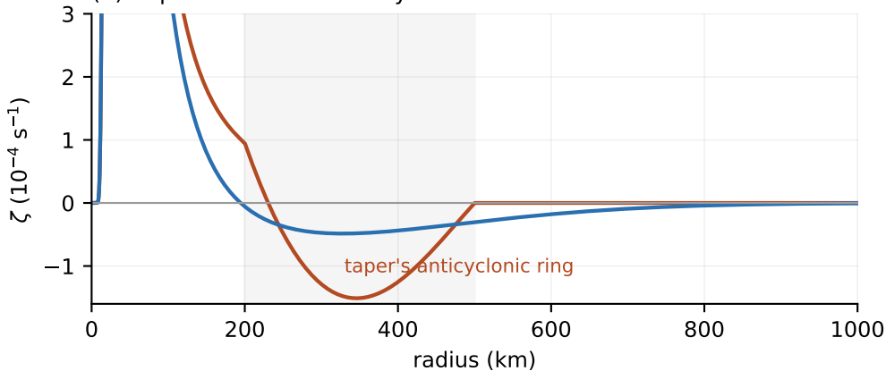
(b) implied relative vorticity
