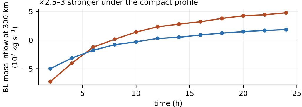
(b) the mechanism: mid-radius Ekman inflow, \times 2.5 –3 stronger under the compact profile
