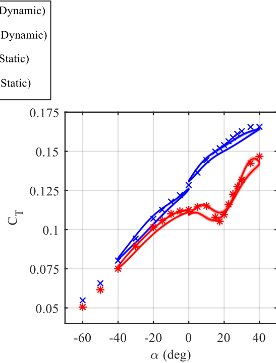
Fig. 21 Dynamic data for f = 0.6 Hz, J = 0.47 , amplitude of 20 degrees, and d = 3.1R .
