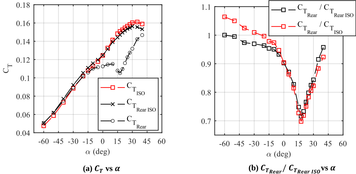
Fig. 14 Rear propeller thrust coefficient for J = 0.47 at d = 3.1R .
