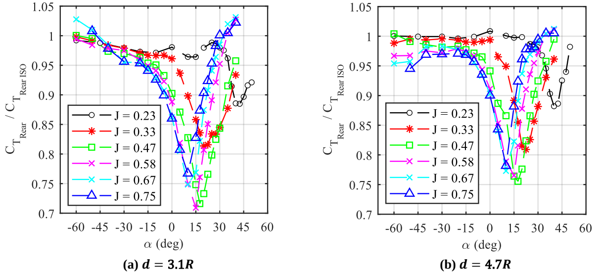
Fig. 17 C_{T_{Rear}}/C_{T_{Rear ISO}} versus \alpha for different advance ratios.
