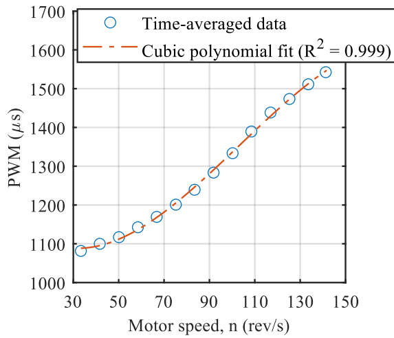
Fig. 7 Steady state motor PWM versus n for wind-off conditions at 30 Volts.
