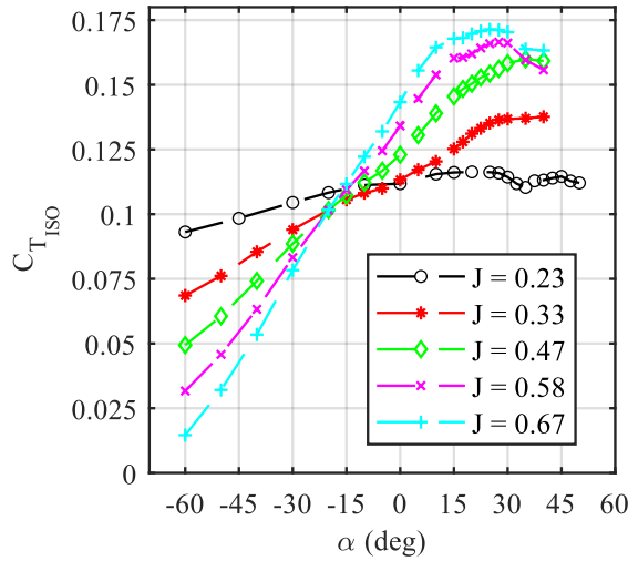
Fig. 9 C_{T_{ISO}} versus \alpha for J \in [0.23, 0.67] .
