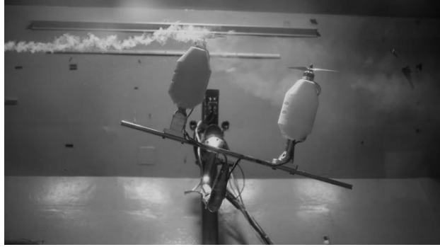
(d) \alpha = 15^\circ , C_{T_{Rear}} / C_{T_{Rear ISO}} = 0.74
