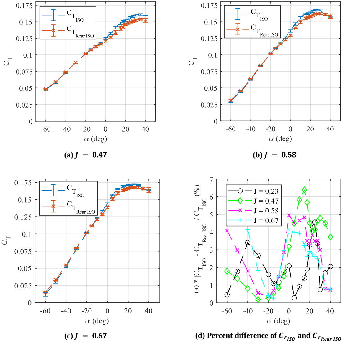
Fig. 13 Comparison of rear propeller thrust coefficients between phase one and two of testing.
