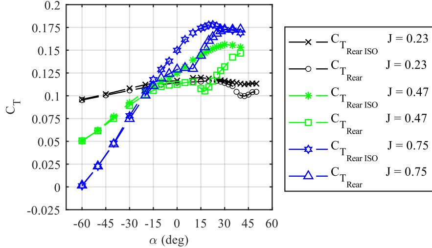
Fig. 16 C_{T_{Rear ISO}} and C_{T_{Rear}} versus \alpha for different advance ratios at d = 3.1R .
