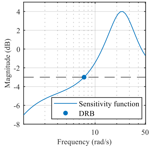
Fig. 8 Magnitude plot of sensitivity function and DRB of the closed-loop system.
