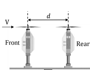
Fig. 2 Side view rendering of tandem configuration at different hub separation distances ( d ) at \alpha = 0^\circ .
