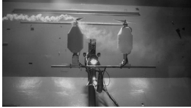
(a) \alpha = 0^\circ , C_{T_{Rear}} / C_{T_{Rear ISO}} = 0.90
