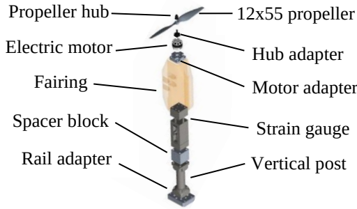
Fig. 1 Isolated propeller assembly.
