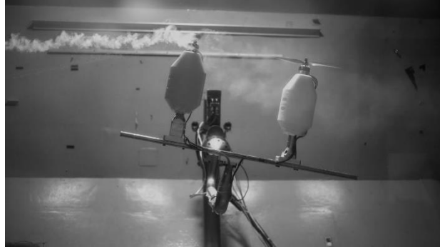
(c) \alpha = 10^\circ , C_{T_{Rear}} / C_{T_{Rear ISO}} = 0.83
