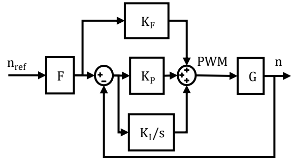
Fig. 6 Block diagram of motor speed control system.
