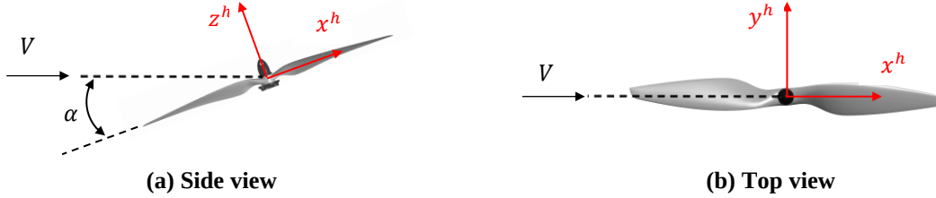
Fig. 10 Hub coordinate system.
