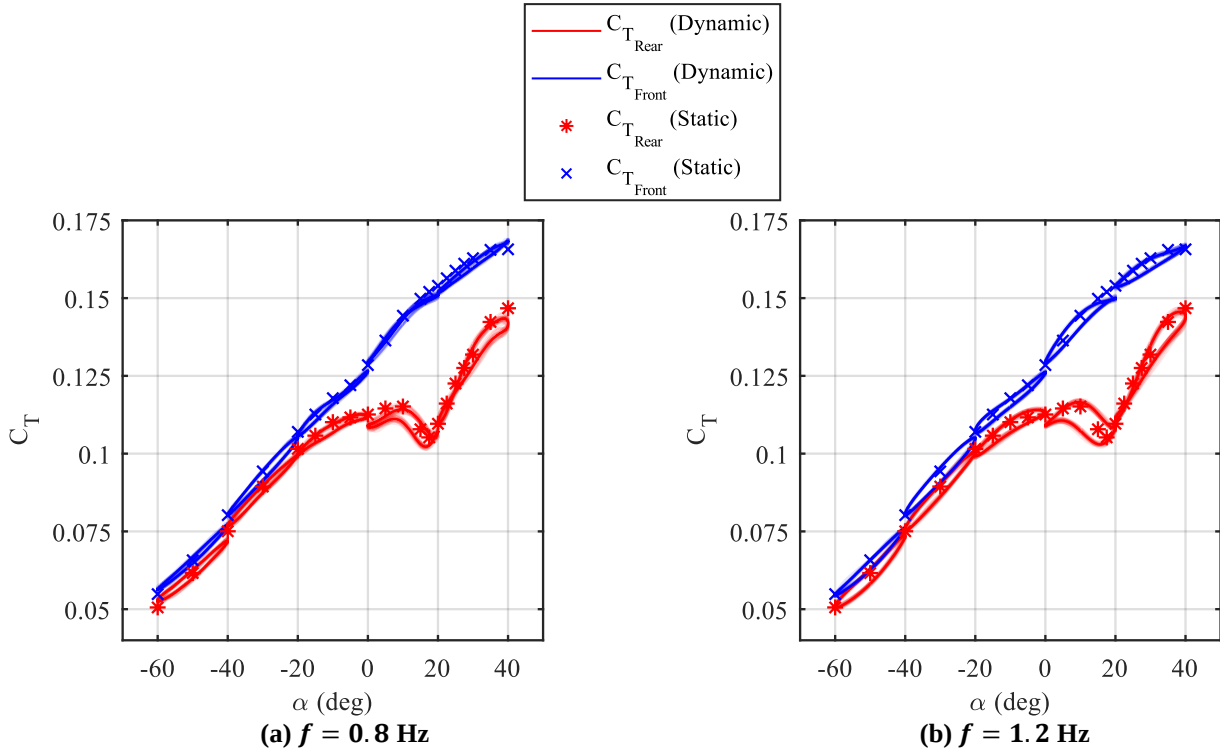
Fig. 19 Hysteresis loops of thrust coefficient at an oscillation amplitude of 10 degrees, J = 0.47 , d = 3.1R .
