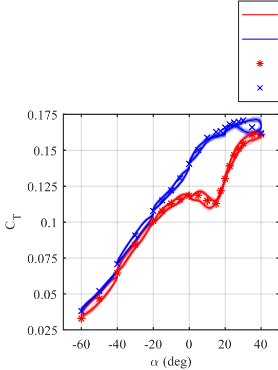
Fig. 20 Dynamic data for f = 1.2 Hz, J = 0.58 , amplitude of 10 degrees, and d = 3.1R .
