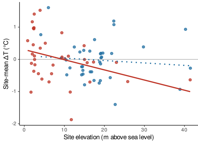
(a) Site-mean \Delta T against elevation
