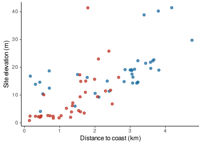
(b) Elevation against distance to the coast
