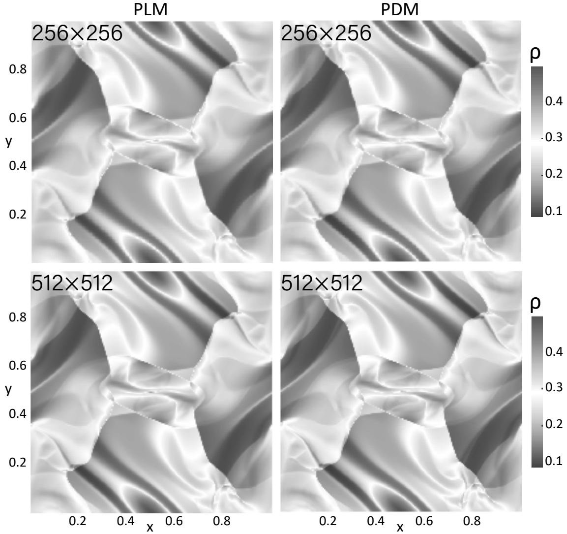
Figure 7. Shown here is the spatial distribution of plasma density of Orszag–Tang simulations at t = 0.5 using different reconstructions and resolutions: 256 \times 256 (top) and 512 \times 512 (bottom), piecewise linear method (left) and partial donor cell method (right).
