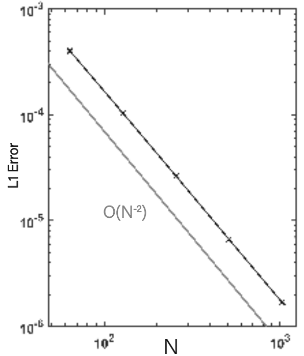
Figure 5. Shown here is the convergence of the nonlinear polarized Alfvén waves test.
