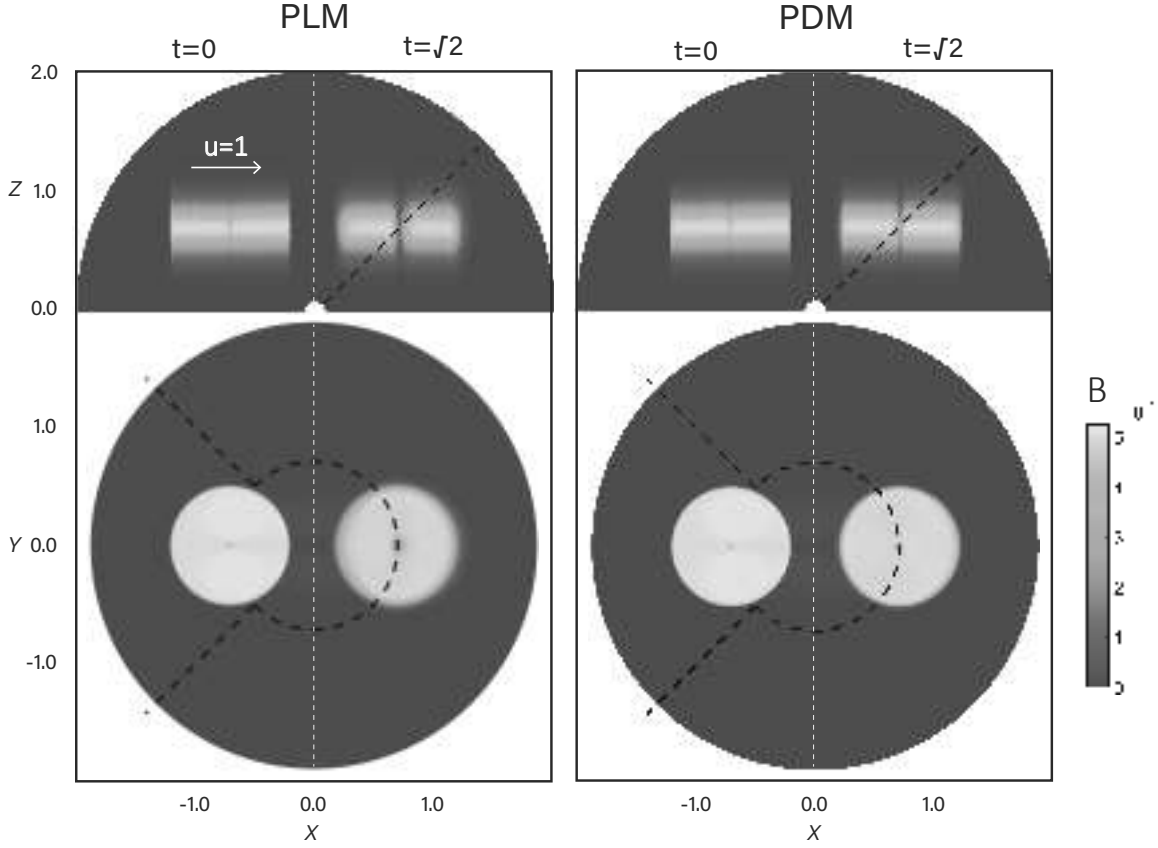
Figure 10. Shown here is the magnetic field in 3D magnetic field-loop advection test in spherical coordinate at t = \sqrt{2} . The top panels show vertical slices through the y = 0 plane, and the bottom panels show horizontal slices through the z = \sqrt{2}/2 plane. The black dashed lines represent the Yin–Yang boundaries. The left panel shows the results obtained with PLM reconstruction, and the right panel shows the results obtained with PDM reconstruction.
