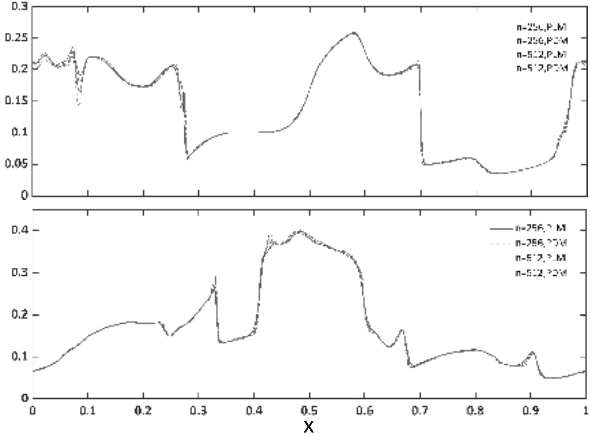
Figure 8. Shown here is the line profiles of plasma pressure at y = 0.3125 (top) and y = 0.4277 (bottom) from four Orszag–Tang simulations at t = 0.5 . The results are shown for 256 \times 256 grid (red line) and 512 \times 512 grid (blue line), PLM reconstruction (solid line) and PDM reconstruction (dashed line).
