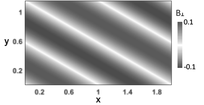
Figure 4. Shown here is the spatial distribution of B_{\perp} of nonlinearly circularly polarized Alfvén waves after propagating one wavelength, using the PLM and a grid of 256 \times 256 cells.
