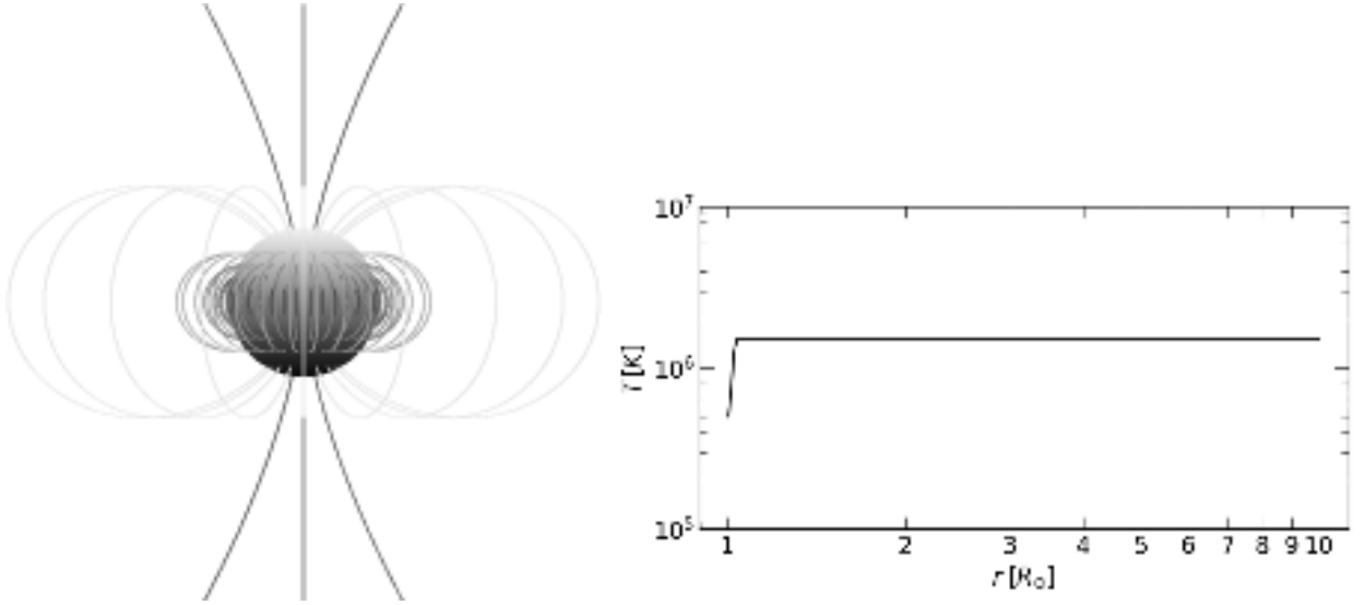
Figure 11. Shown here is the initial dipole magnetic field lines (left) and the initial temperature profile for the 1D hydrostatic corona (right). The gray scale on the sphere in left panel shows the dipolar normal magnetic field distribution B_r on the solar surface.
