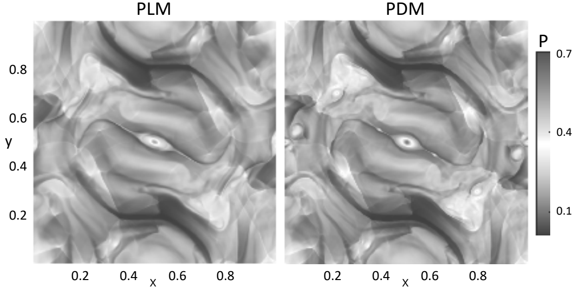
Figure 9. Shown here is the spatial distribution of plasma pressure of Orszag–Tang simulations at t = 1 using a 512 \times 512 grid: results obtained with PLM (left) and PDM (right).
