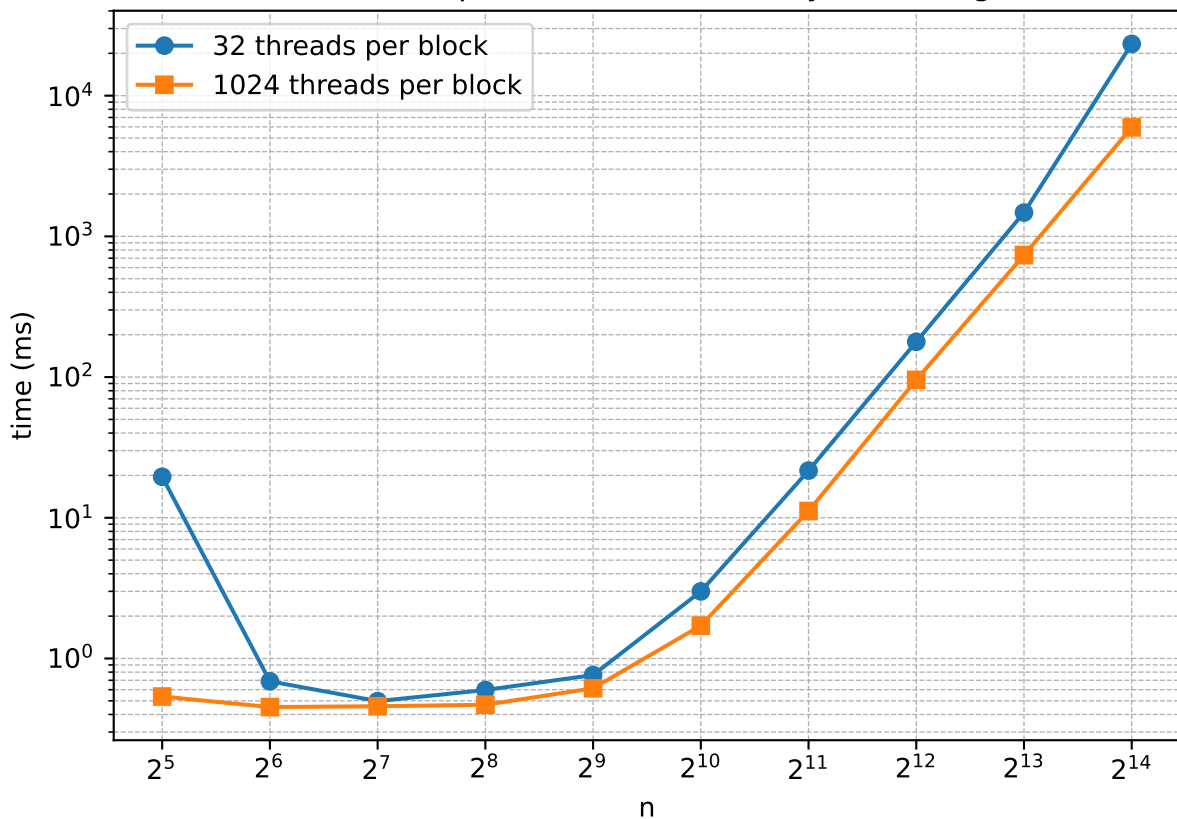
Matrix Multiplication Time vs Array Side Length
