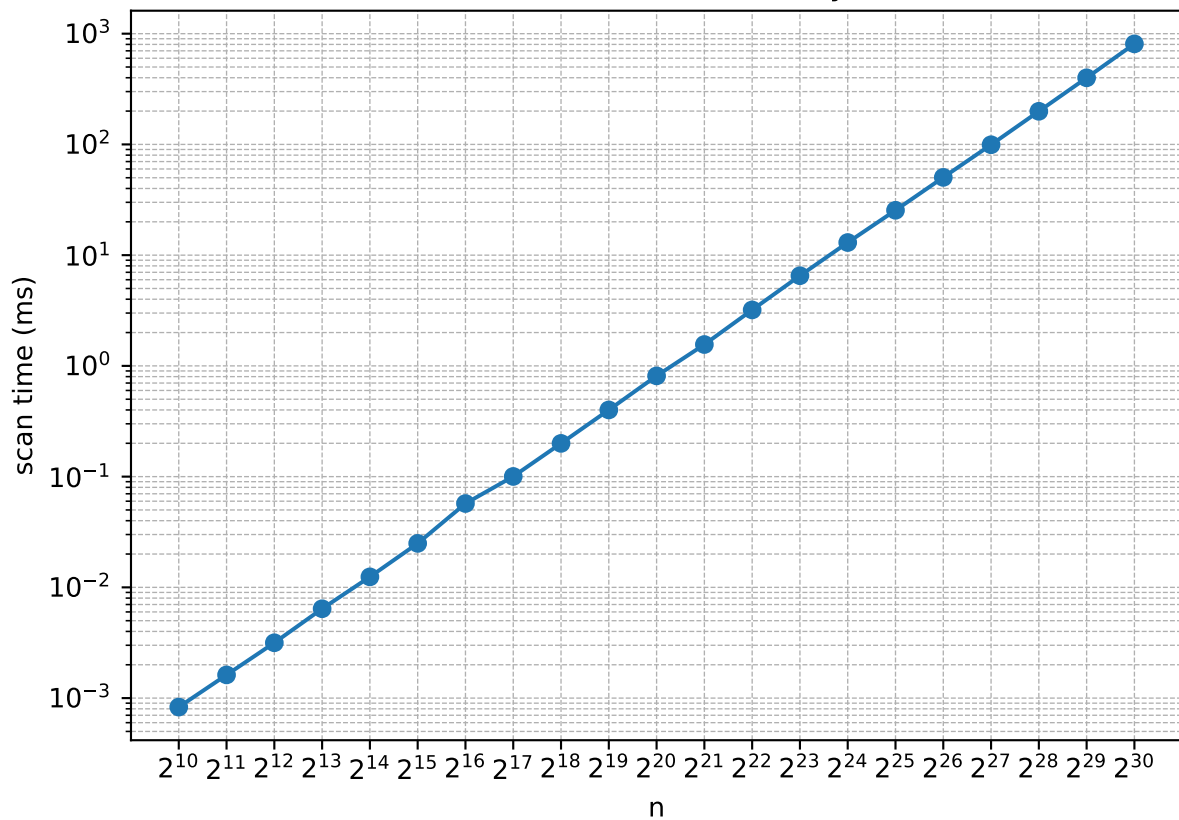
Inclusive Scan Time vs Array Size
