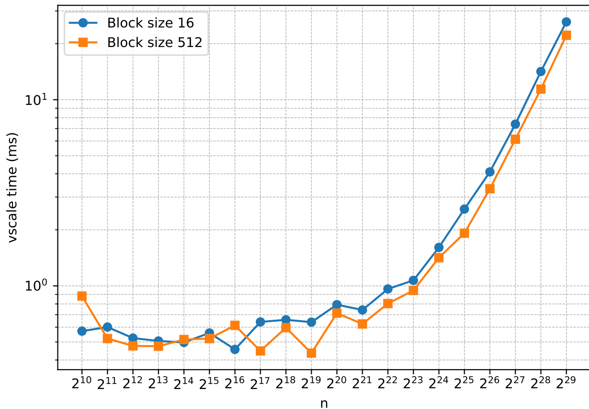
vscale time vs n for different block sizes
