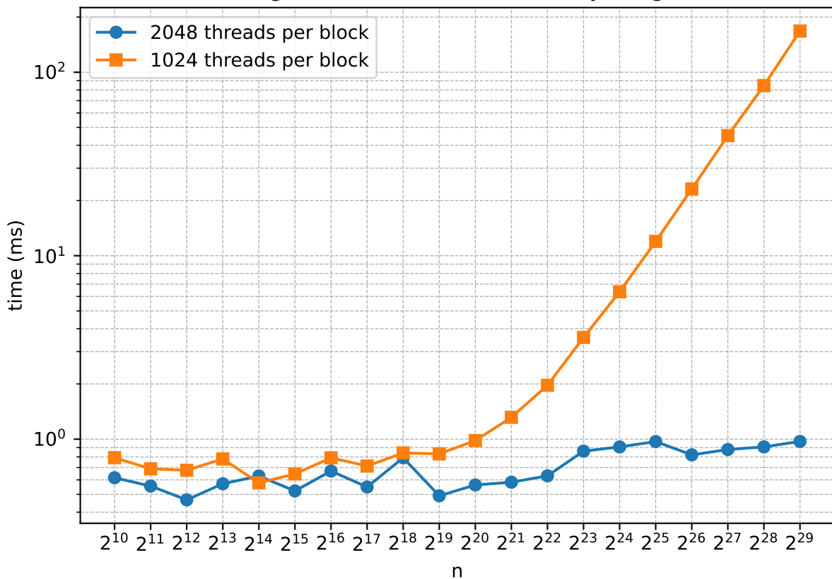
Image Convolution Time vs Array Length
