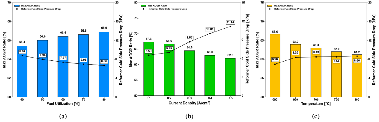
Figure 4: Maximum AOGR ratio permitted for variations in (a) FU_{stack} , (b) j , and (c) T_{stack} .
