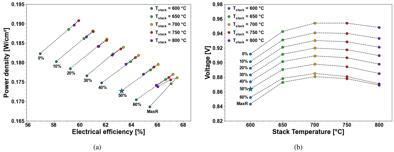
Figure 6: Performance map showing (a) electrical efficiency and power density and (b) voltage as a function of T_{stack} and AOGR ratio. The blue, green, yellow, red, purple markers represent T_{stack} condition of 600, 650, 700, 750, 800 °C, respectively. Number labels on the markers represent AOGR ratio, and the star marker represents base case operation.
