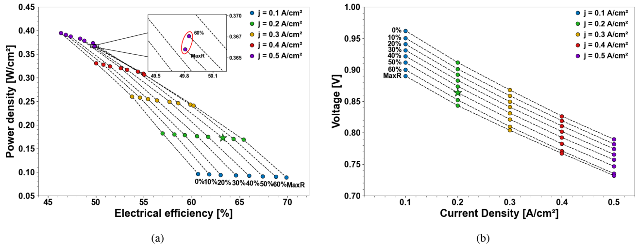
Figure 5: Performance map showing (a) electrical efficiency and power density and (b) voltage as a function of j and AORR ratio. The blue, green, yellow, red, purple markers represent j condition of 0.1, 0.2, 0.3, 0.4, 0.5 A/cm², respectively. Number labels on the markers represent AORR ratio, and the star marker represents base case operation.
