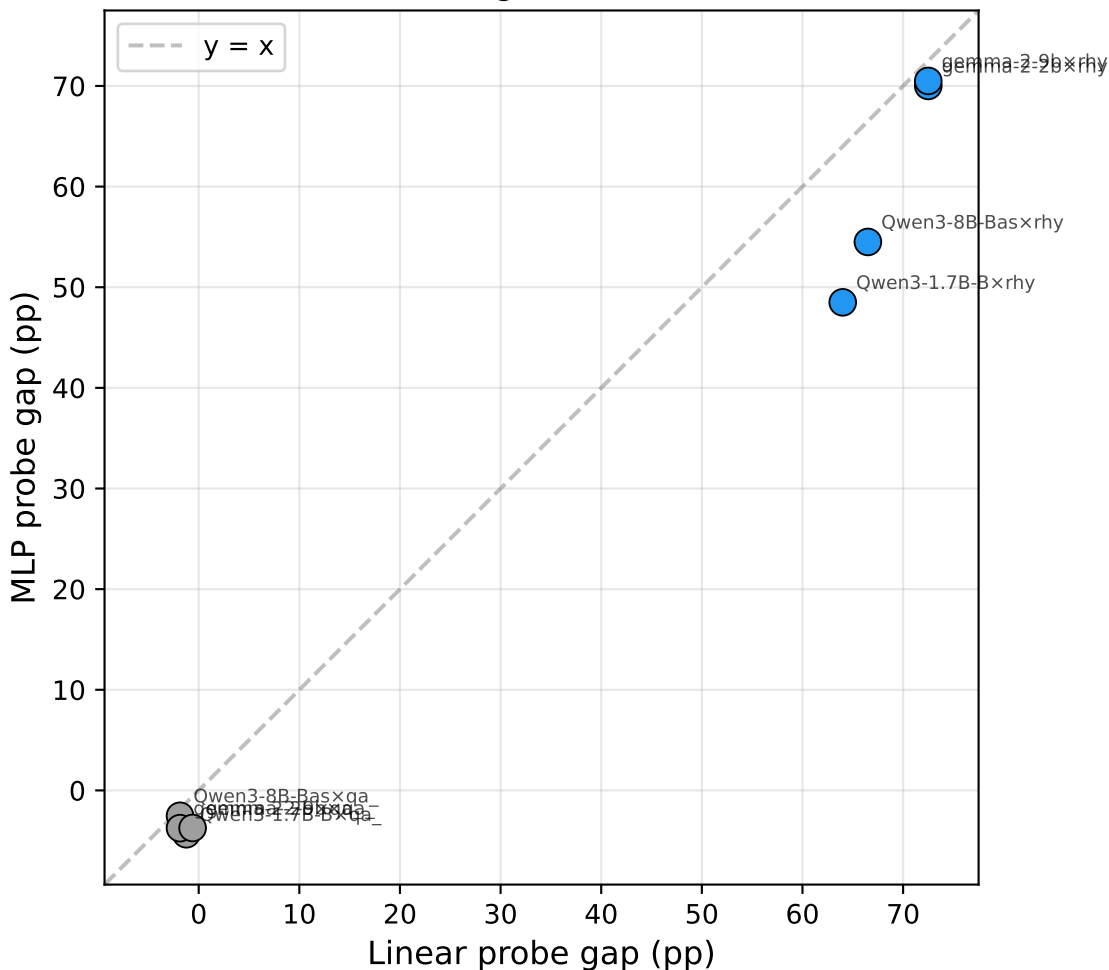
MLP vs Linear probe: 8/8 agree on sign (Hewitt & Liang robustness check)
