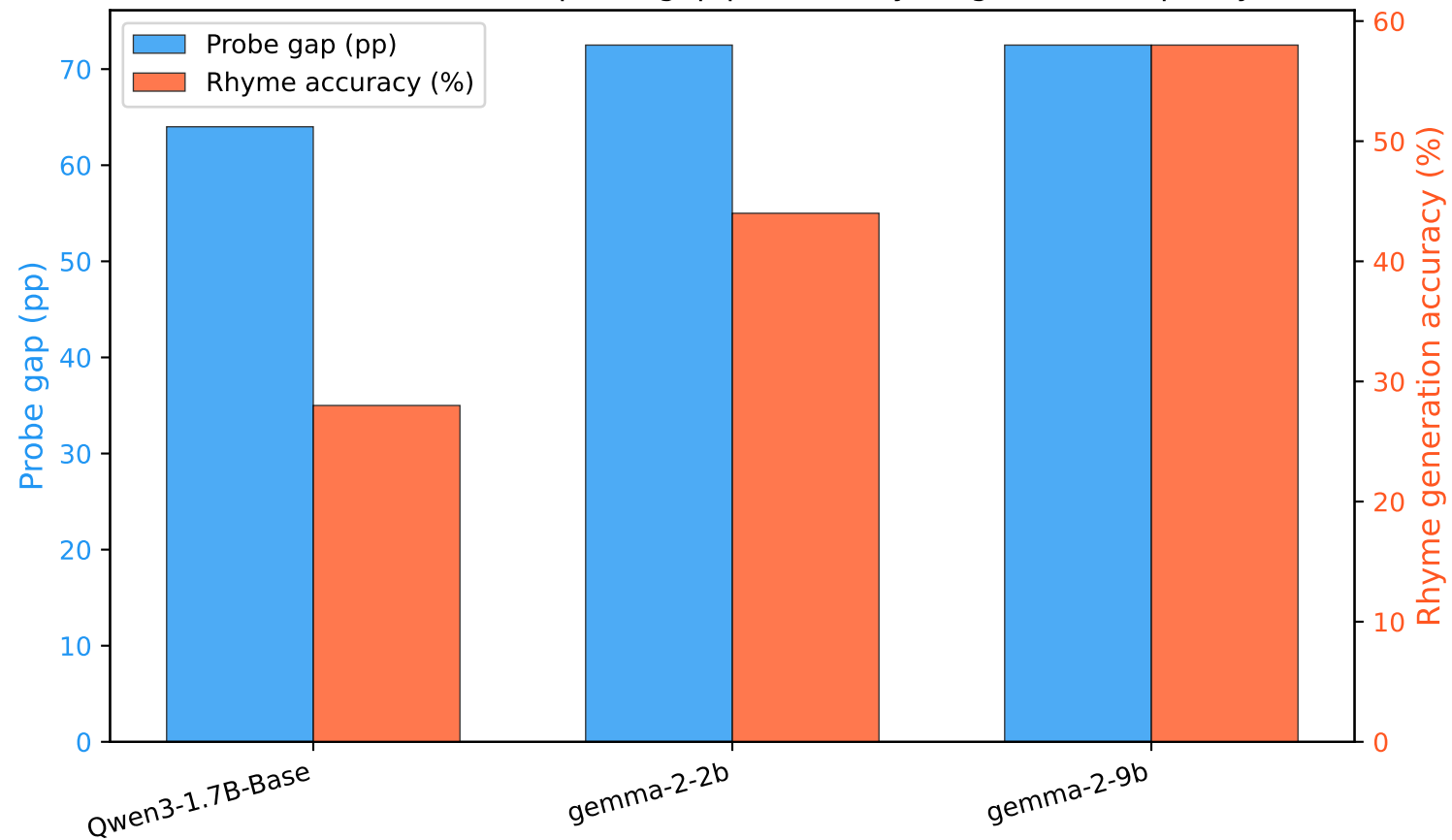
Behavioral validation: probe gap predicts rhyme generation quality
