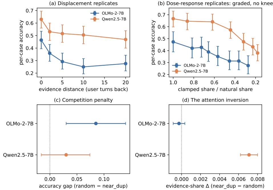
Figure 7: The causal program replicates on Qwen2.5-7B, except competition. (a) The distance ladder at matched fill ( n=192/\text{arm} in both families). (b) The share \rightarrow accuracy dose-response, x as a fraction of each family’s natural share (OLMo layer-24-indexed, common subset n=131 ; Qwen all-layer, n=181 – 192 ): graded with no knee in both. (c) The competition contrast is significant on OLMo, not detected on Qwen. (d) The evidence’s attention under near-duplicate context: flat on OLMo, rising on Qwen, with disjoint intervals—the family divergence. Whiskers in (a, b) are per-point Wilson 95% intervals; (c, d) show the paired bootstrap CIs quoted in the text.
