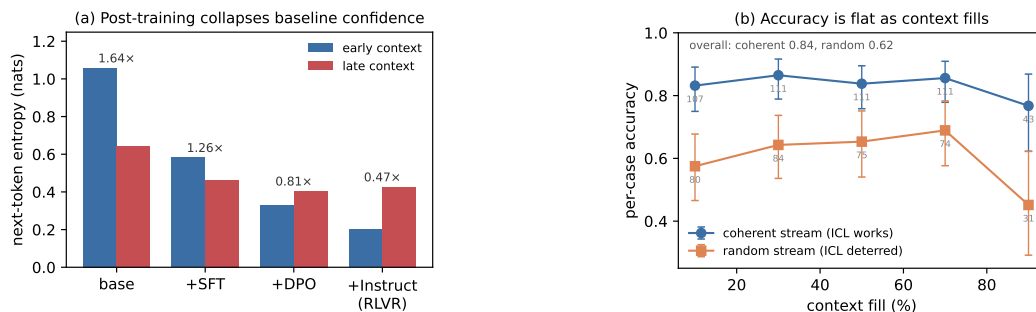
Figure 6: Signature details. (a) OLMo-2’s post-training chain collapses baseline entropy stage by stage; the within-context ratio falls across stages, so alignment installs a level shift, not a steeper slope. (b) Accuracy is flat with fill in both the coherent and the random-subject stream; the random stream is lower throughout (harder subjects), not sloped. Error bars are Wilson 95% intervals with per-bin n printed; the final bins are the smallest ( n=31/43 ) and their intervals overlap the preceding bins’, so the endpoint movement is not resolved at this n .
