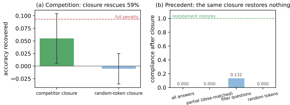
Figure 5: One intervention, opposite outcomes. The same scale-0 generation-time closure (a) recovers 59% of the competition penalty (paired n=365 ; bars are paired accuracy deltas with 95% CIs; dashed line marks the full in-run penalty), but (b) restores no compliance at depth 42 when applied to the demonstrated answer spans ( n=40 /arm; every closure arm sits at or near the eroded floor while restating the instruction restores 1.000). Competition is generation-time reading; the precedent mode is already in place by prefill.
