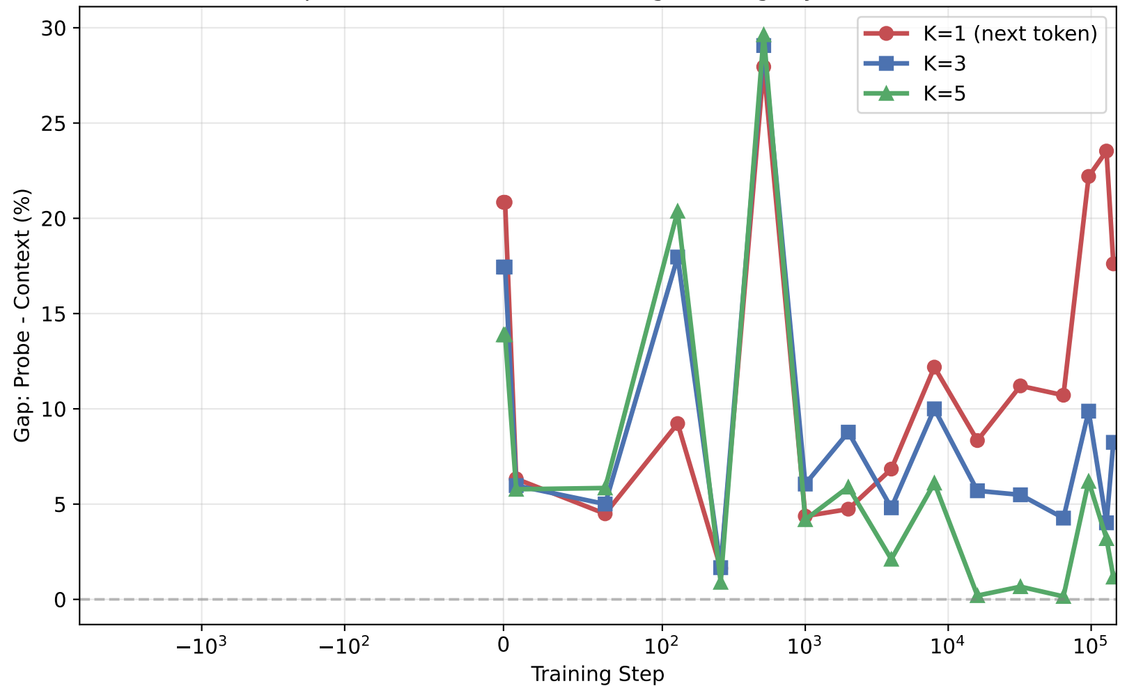
Temporal Horizon Narrows During Training (Pythia-2.8B)
