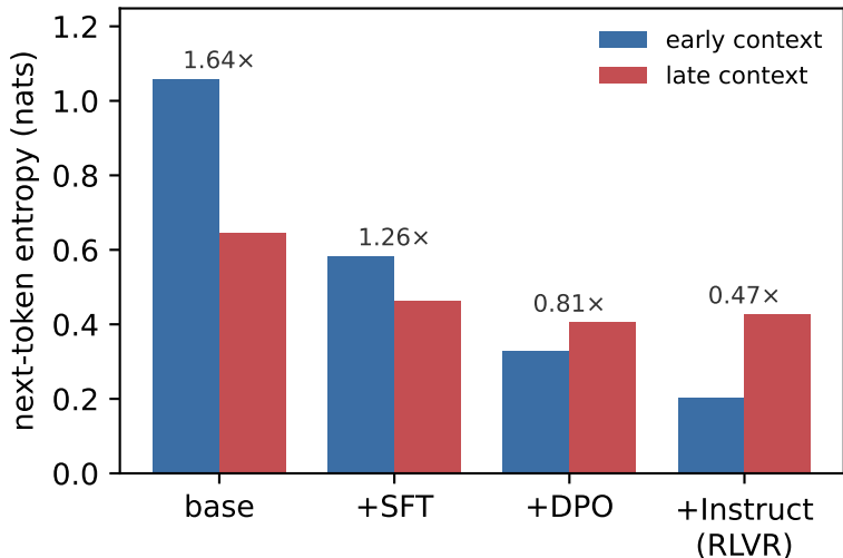
(a) Post-training collapses baseline confidence
