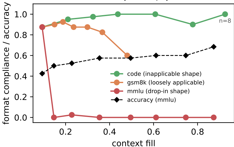
(a) An applicable shape erodes the format; accuracy never pays
