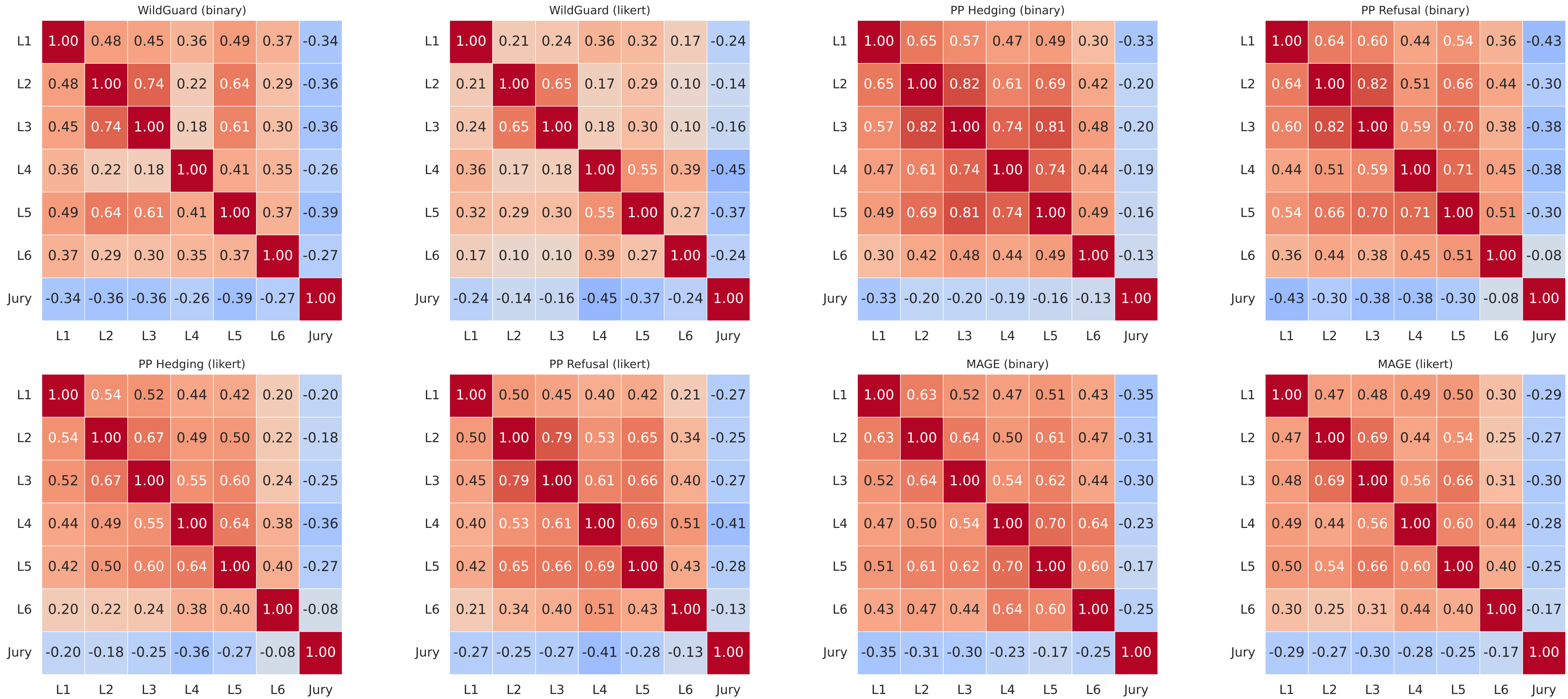
Cross-Level Correlation (example-level, Spearman)
