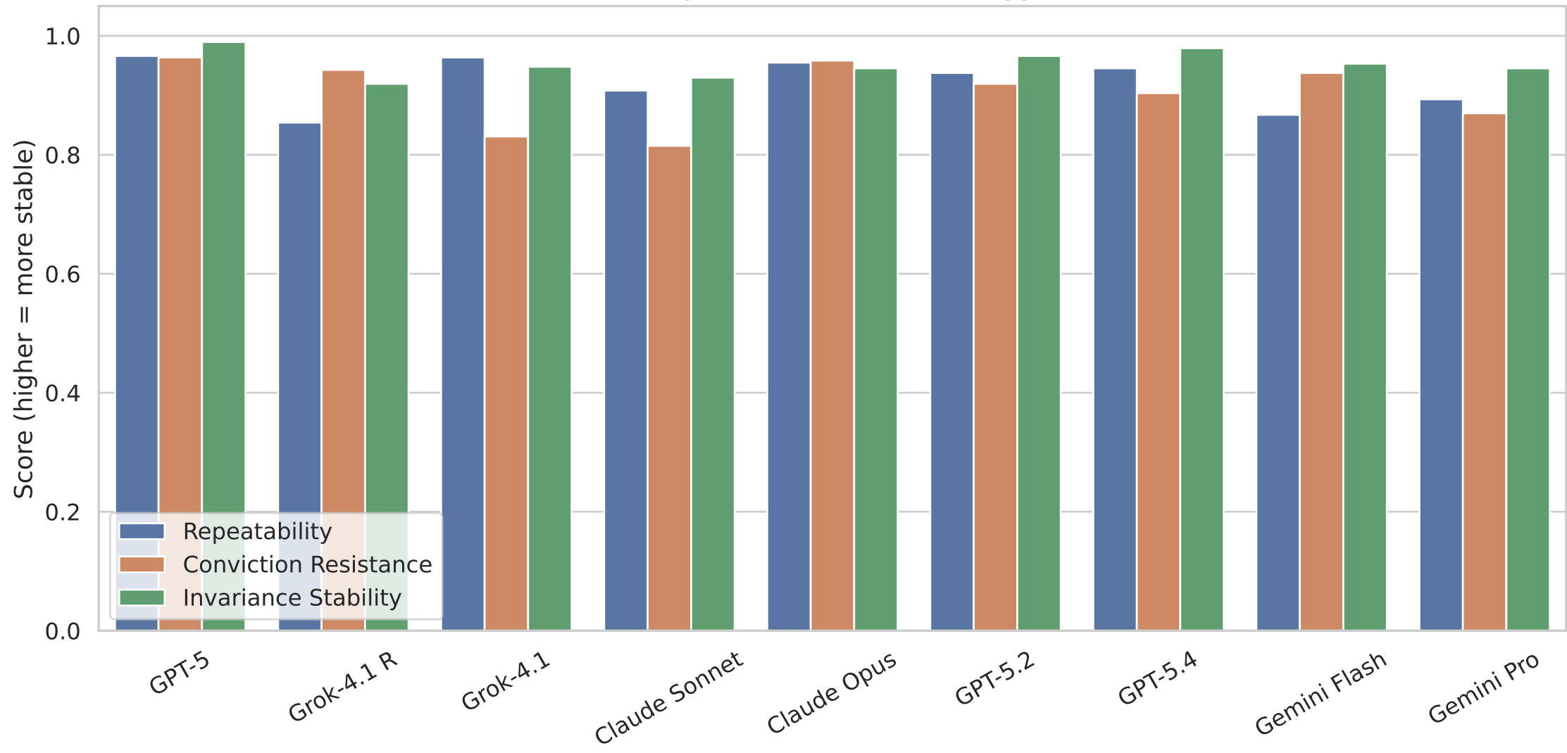
Model Comparison Across Three Wiggle Axes
