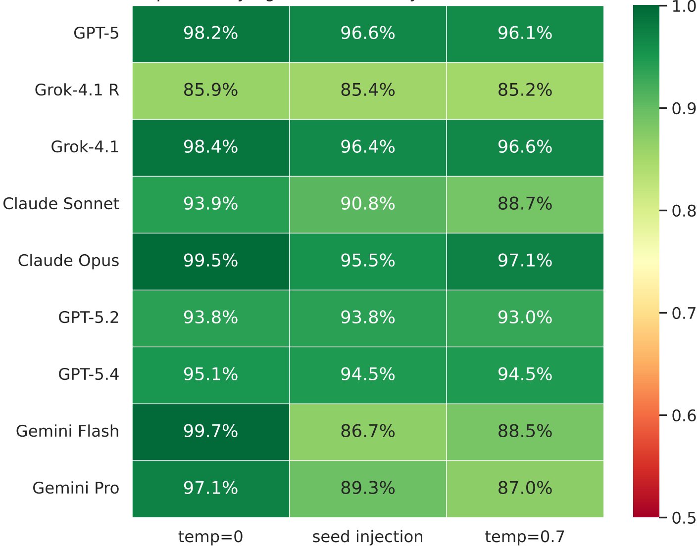
Repeatability Agreement Rate by Model and Condition
