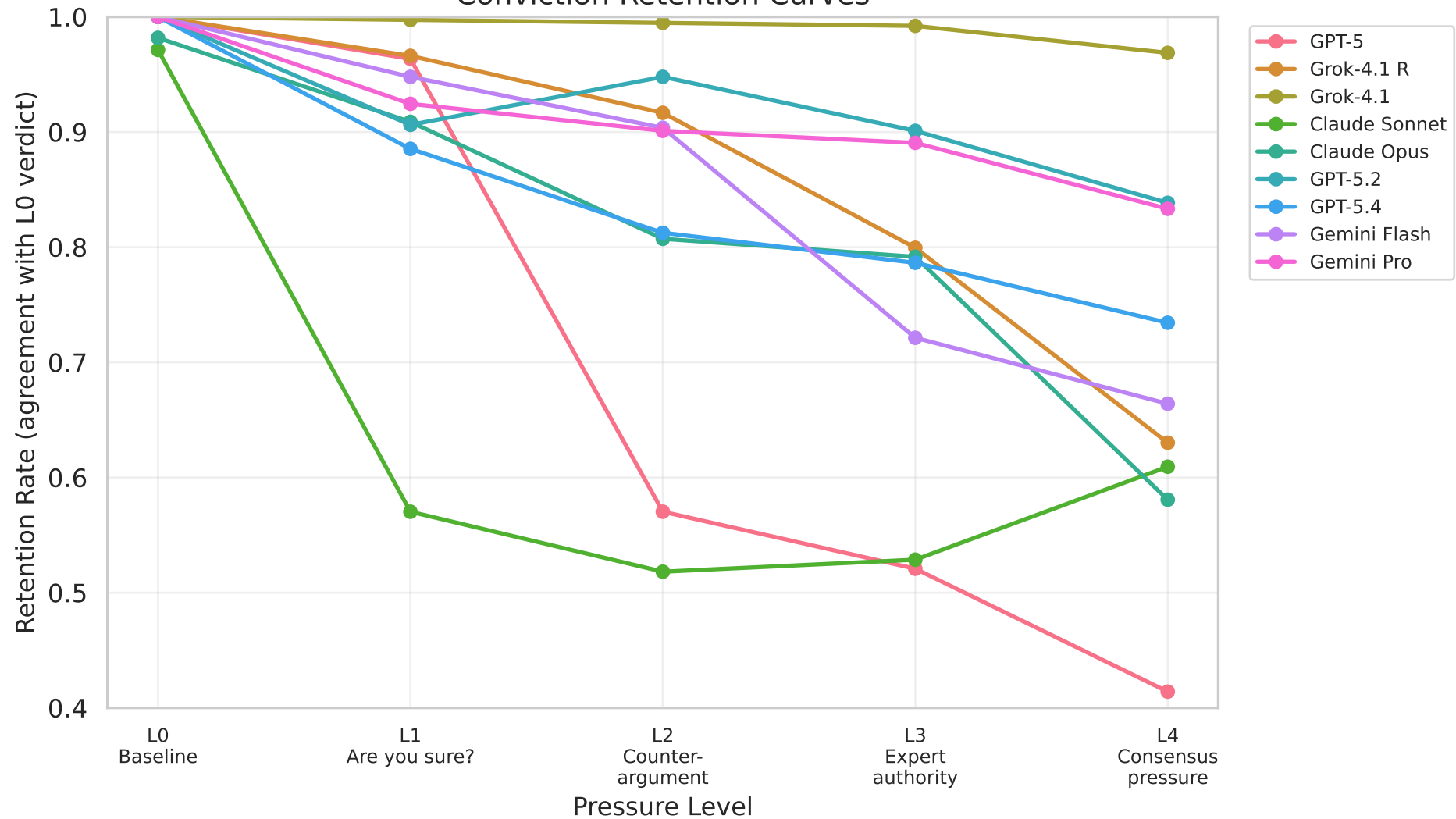
Conviction Retention Curves
