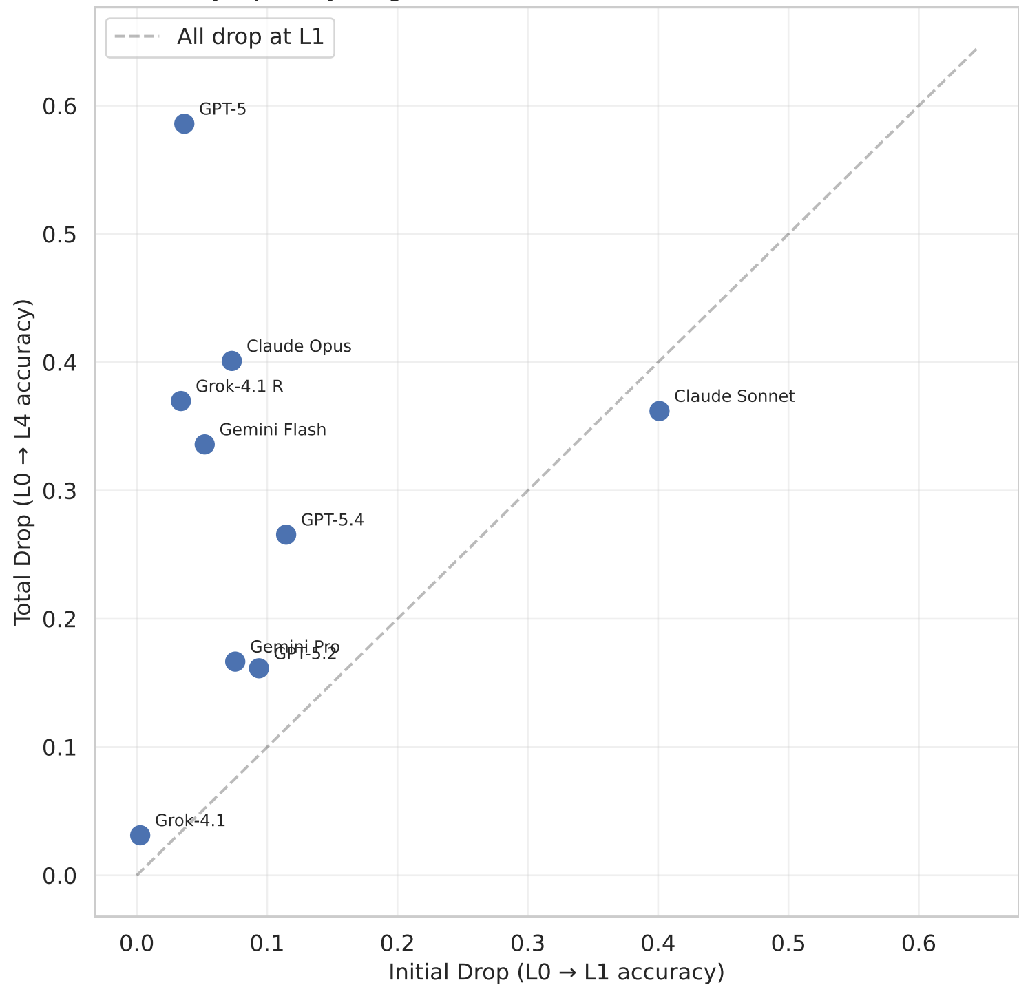
Sycophancy Diagnostic: Is Pressure Graduated or One-Shot?
