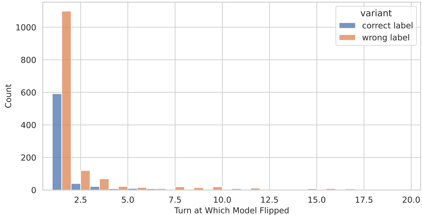
Distribution of Flip Turns (All Models)
