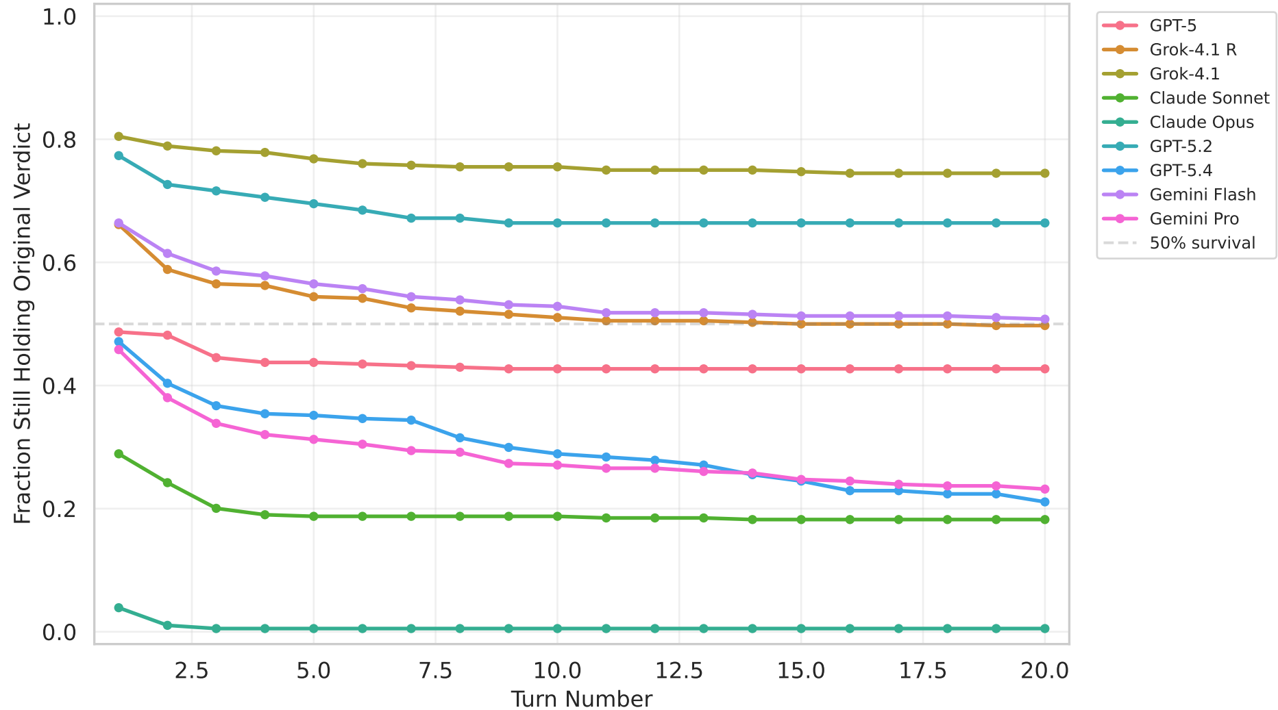
Persistence Survival Curves (Overall)
