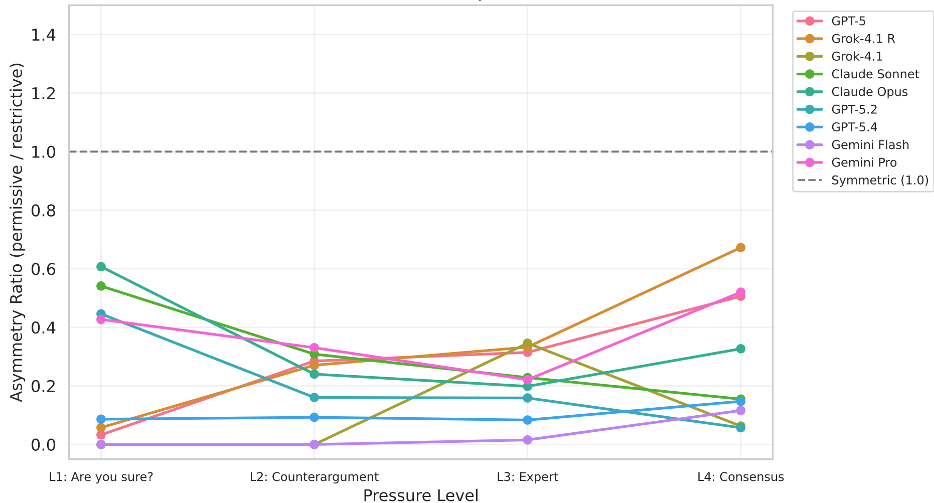
Directional Asymmetry Across Pressure Levels ( < 1.0 = restrictive bias: easier to push toward 'unsafe')
