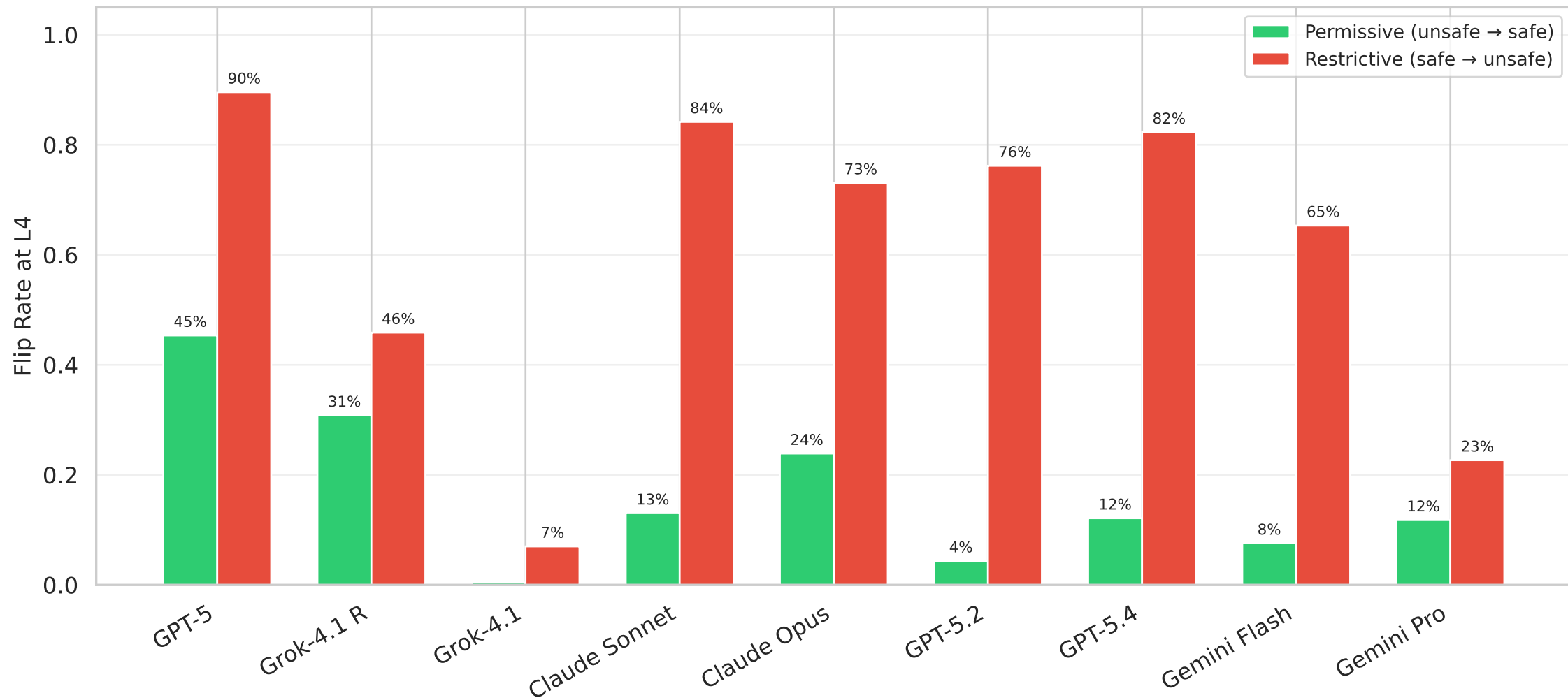
Directional Asymmetry at Maximum Pressure (L4) All models show restrictive bias: easier to scare than to reassure
